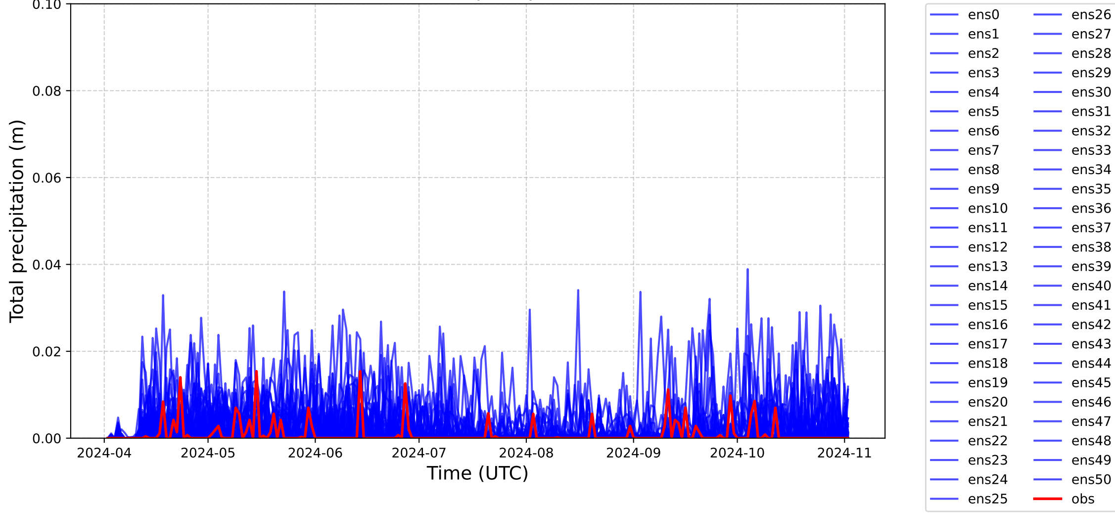
Seasonal forecast (ECSF) and observed total precipitation for FMISID 116859 (2024-04-02)
