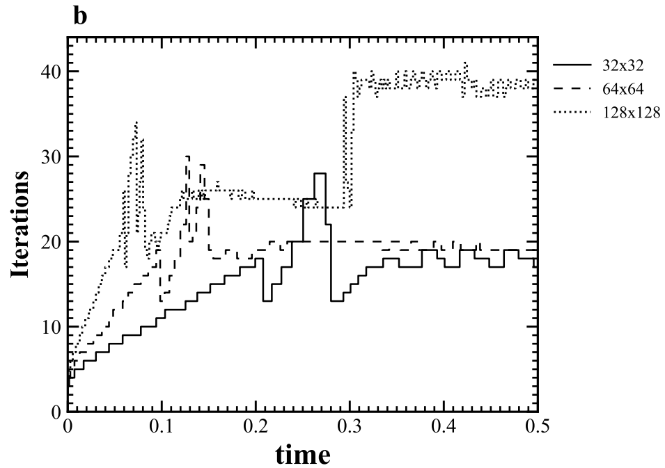
(b) \eta = 0.50
