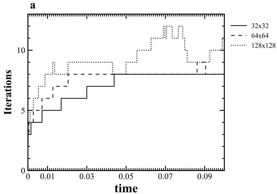
(a) \eta = 0.10
