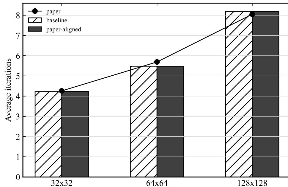
\eta = 0.50 , nonlinear
