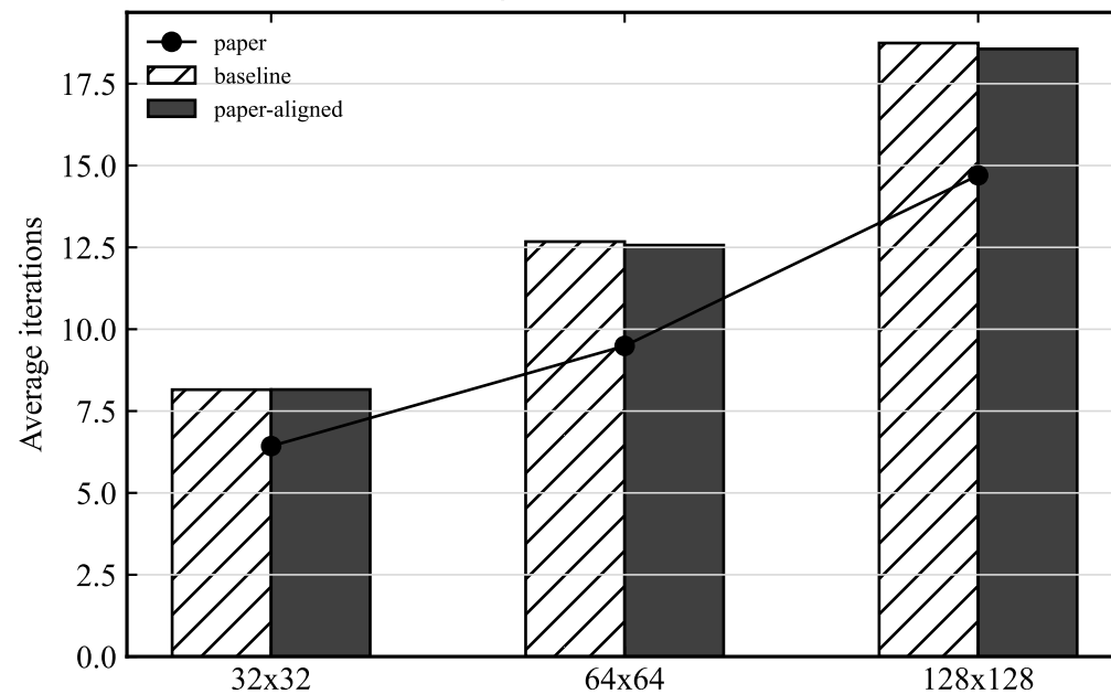
\eta = 0.50 , nonlinear
