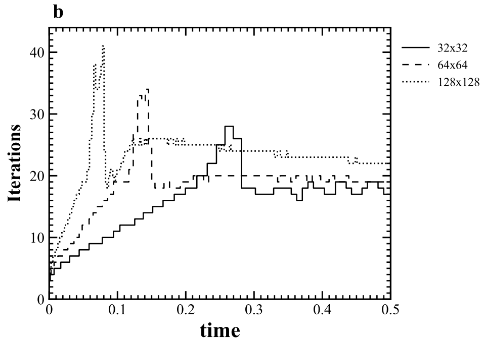
(b) \eta = 0.50
