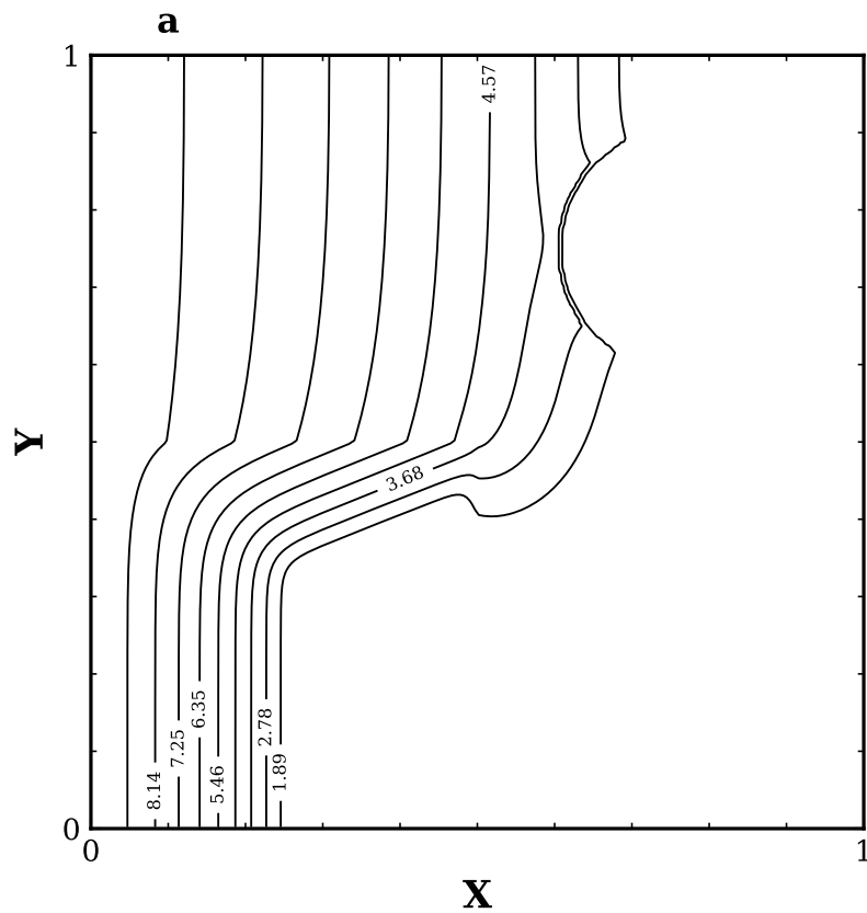
(a) M1, \eta = 0.50 , t = 5
