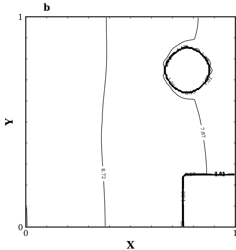
(b) M2, \eta = 0.50 , t = 0.005
