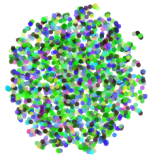
generative model
