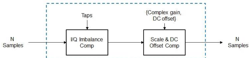
Fig 1: Custom signal conditioning chain for 160MHz
