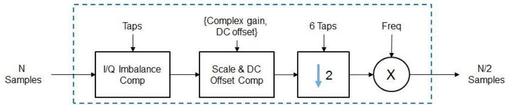
Fig 2: Custom signal conditioning chain for 80MHz
