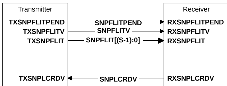
Figure B13.13: SNP channel interface pins
