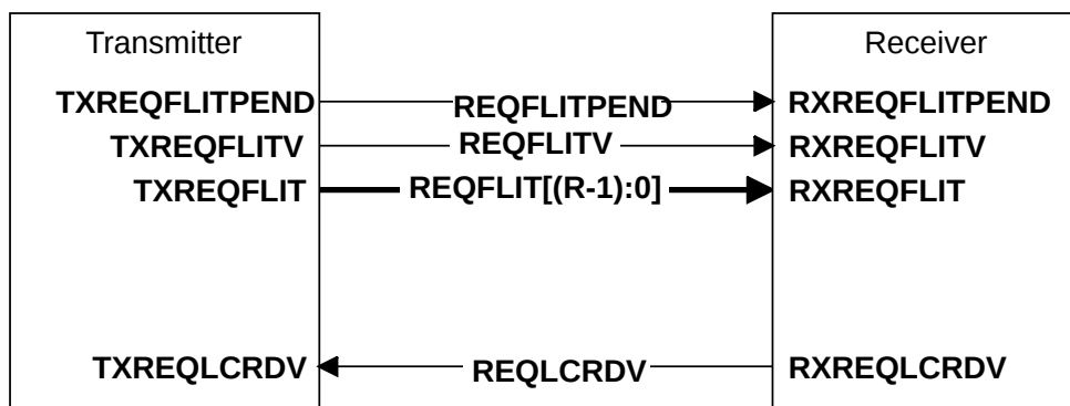
Figure B13.11: REQ channel interface pins
