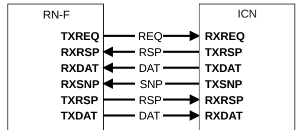
Figure B13.5: RN-F interface
