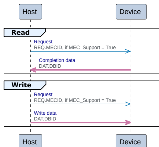
Figure B10.3: RME-CDA fields in host requests to DCM locations
