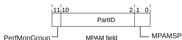
Figure B11.3: MPAM_9_1 subfields bit allocation
