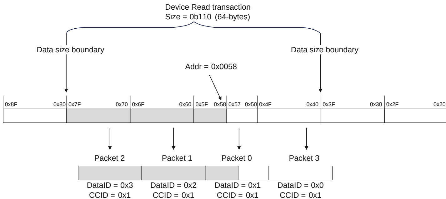
Figure B2.44: Device Read transaction from an unaligned address
