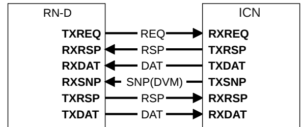
Figure B13.6: RN-D interface
