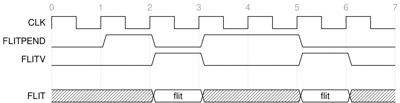
Figure B14.1: FLITPEND indicating a valid flit in next cycle
