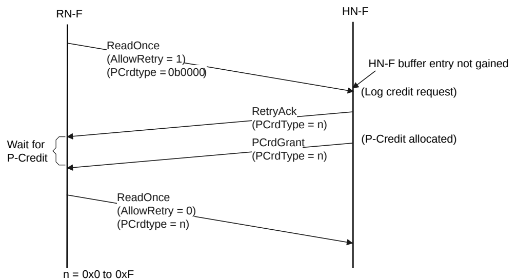
Figure B2.46: Transaction Retry flow
