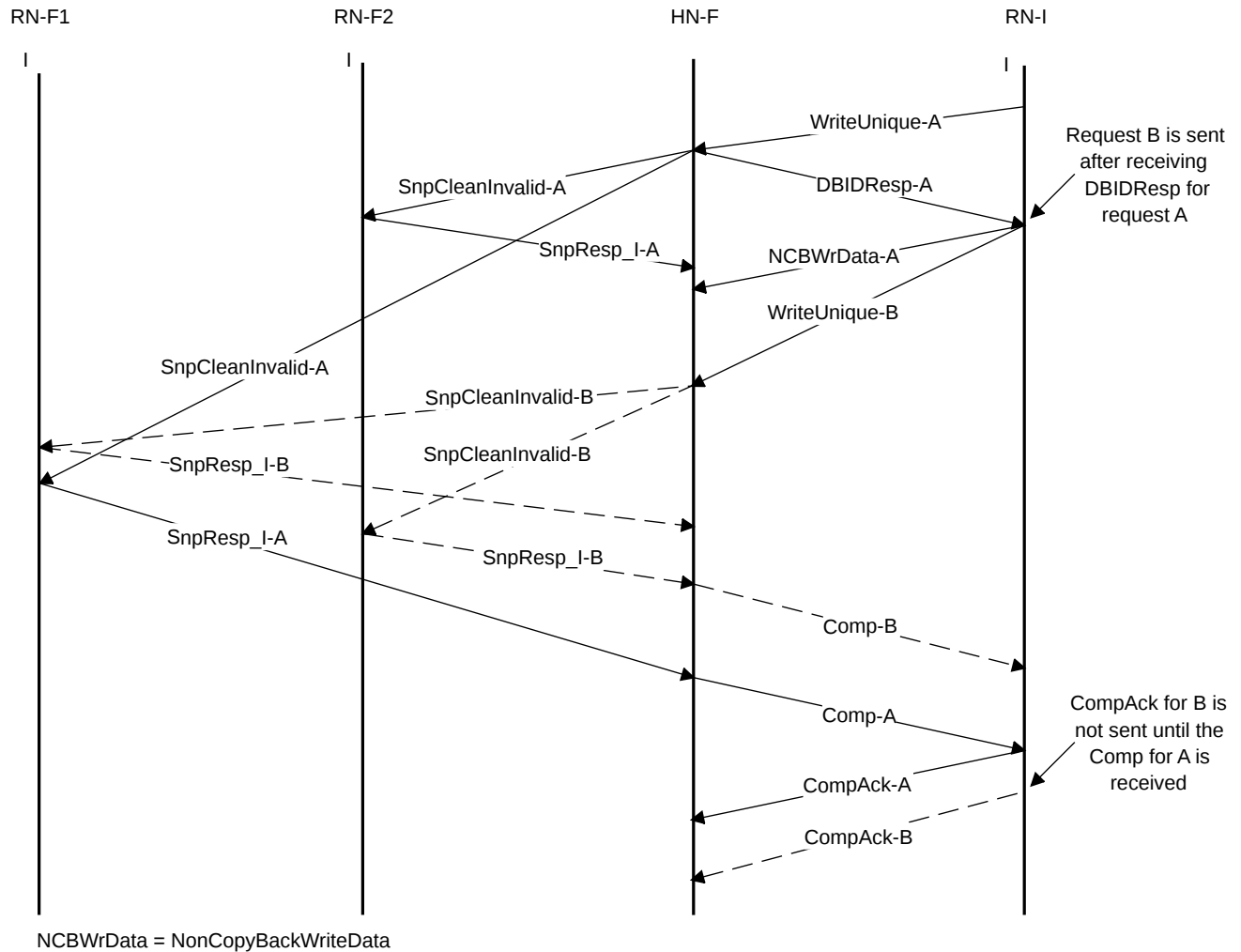
Figure B2.35: Streaming Ordered WriteUnique transactions flow
