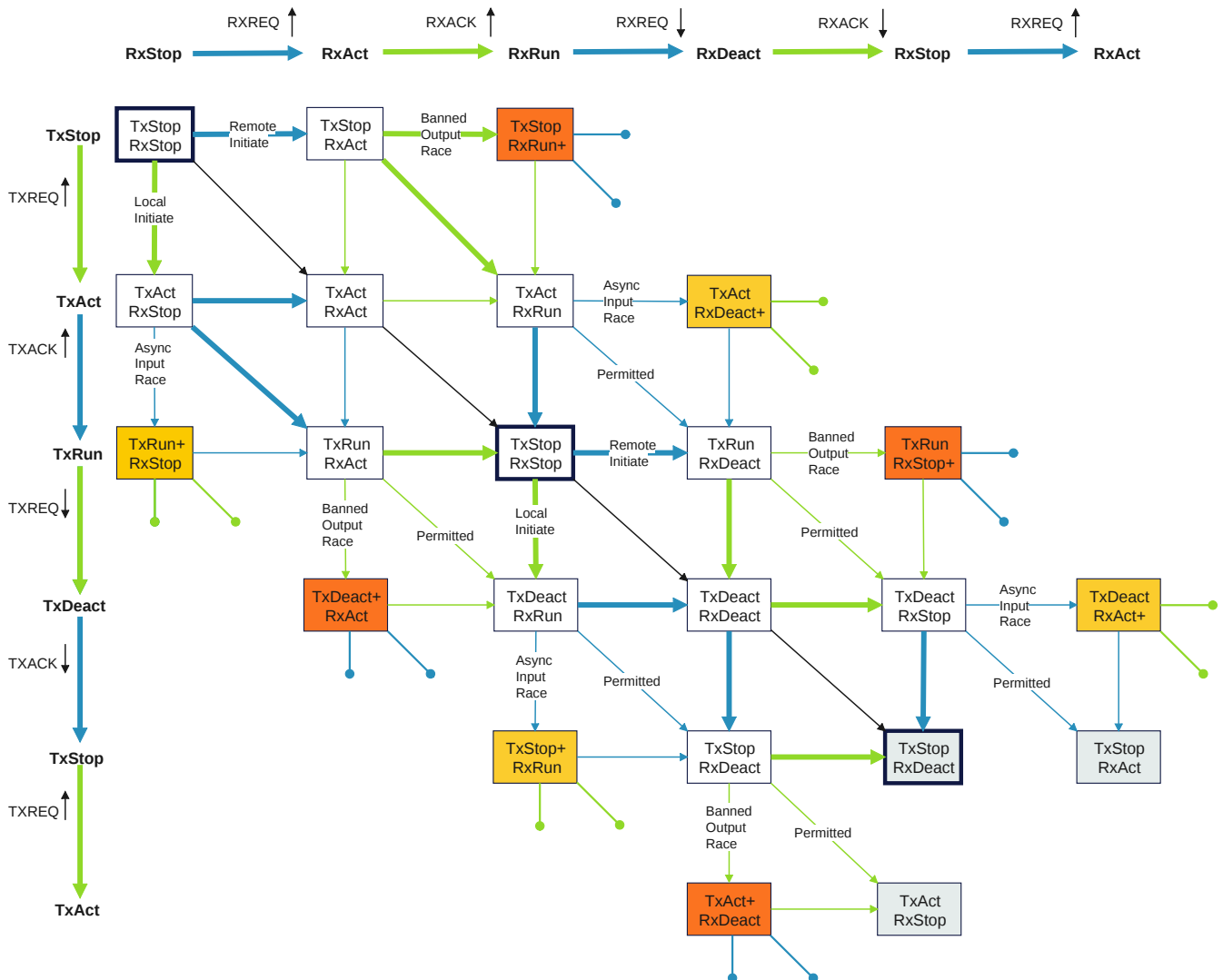
Figure B14.5: Combined Tx and Rx state machines
