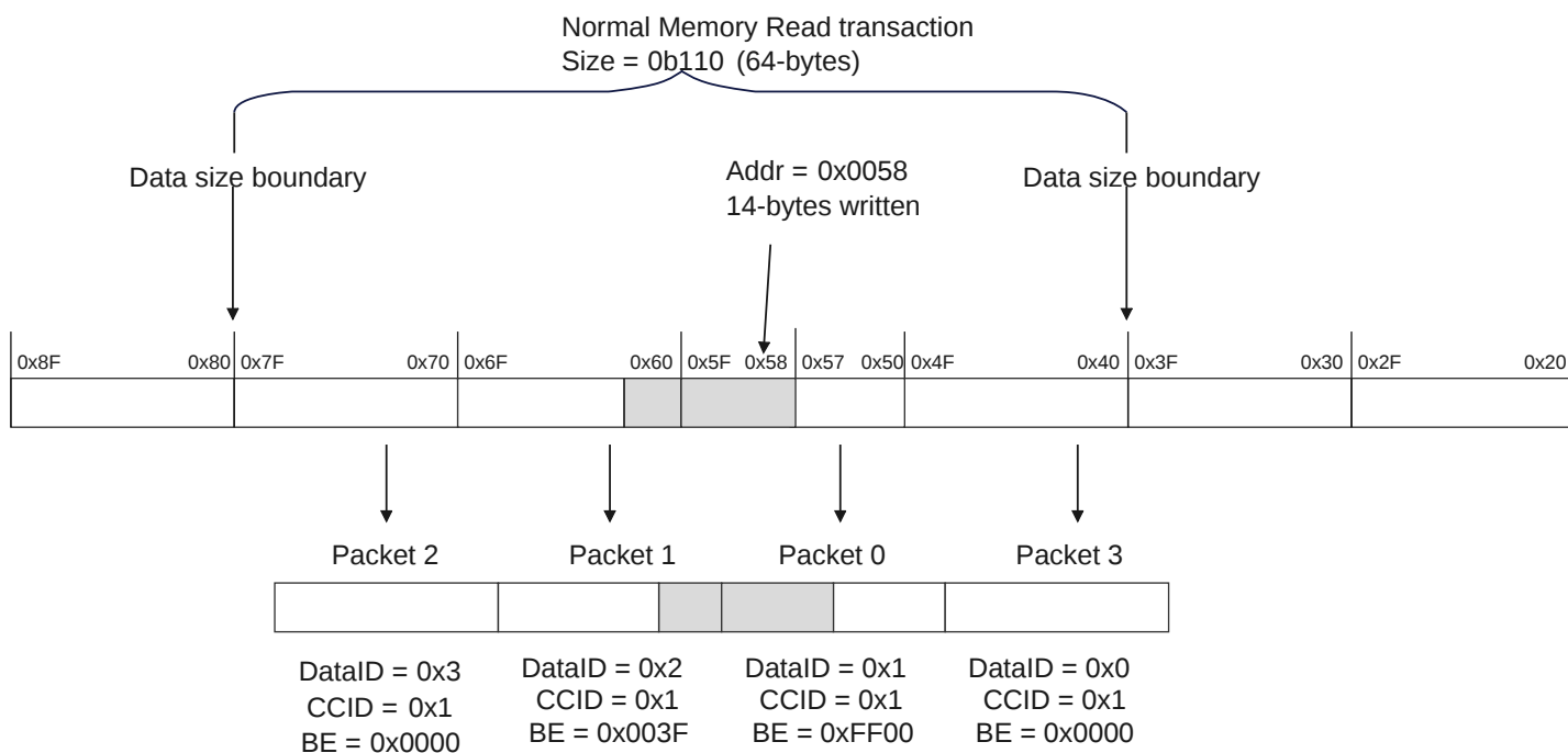
Figure B2.43: Normal memory 14-byte Read transaction from an unaligned address
