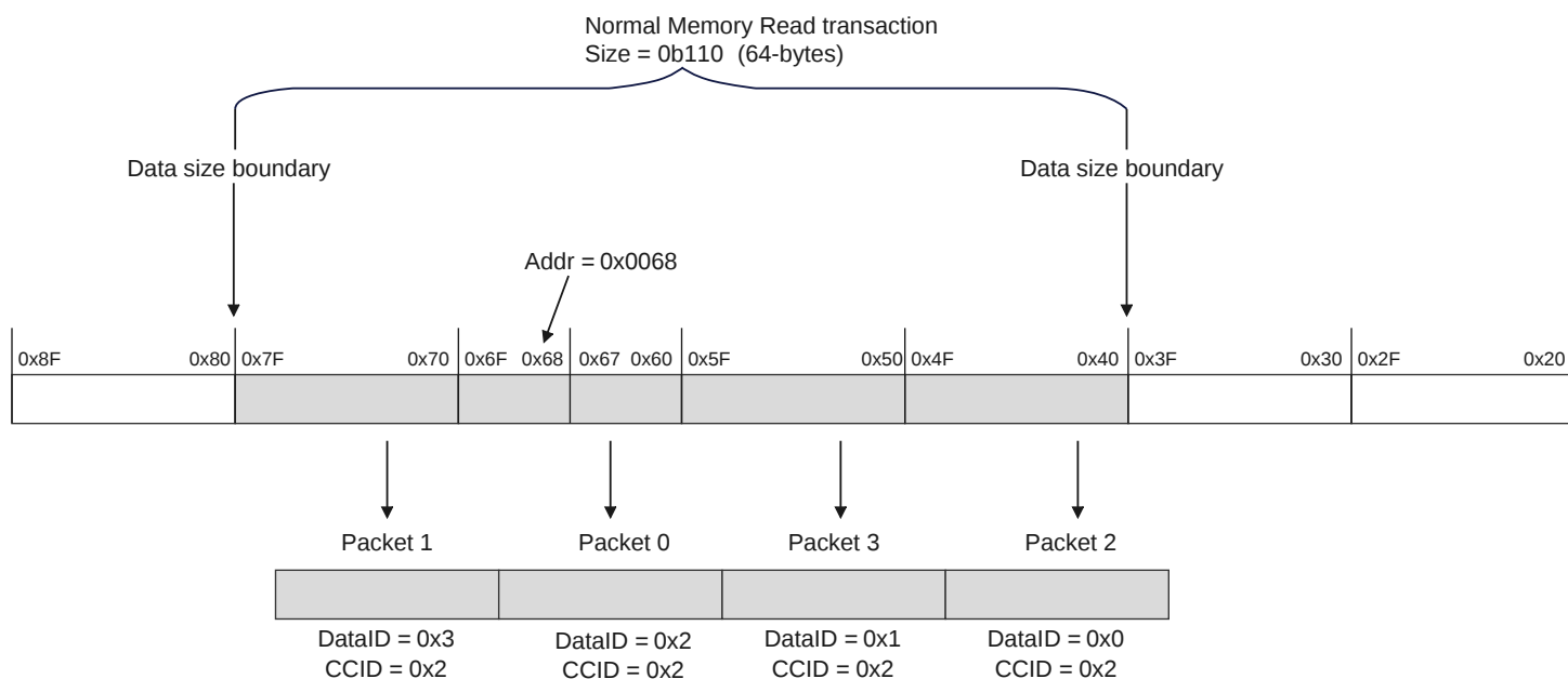
Figure B2.41: Normal memory 64-byte Read transaction from an unaligned address
