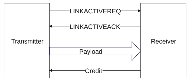
Figure B14.2: Relationship between Payload, Credit, and LINKACTIVE signals
