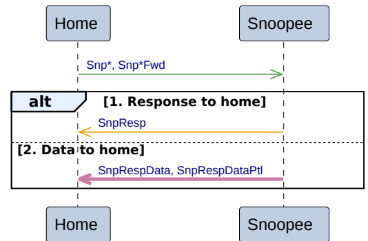
Figure B2.21: Home to Snoopee transactions
