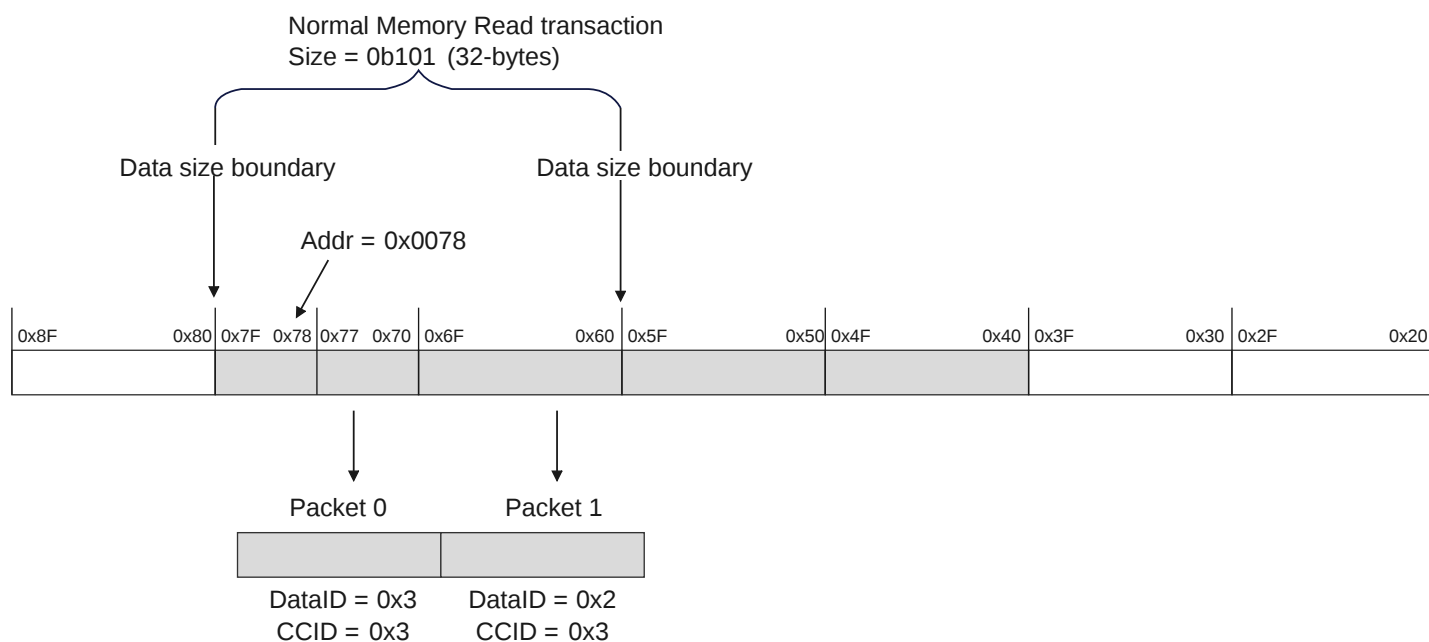
Figure B2.42: Normal memory 32-byte Read transaction from an unaligned address
