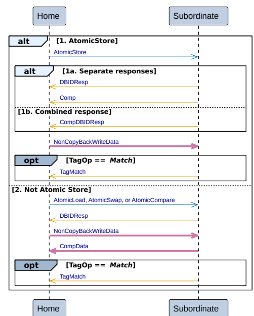
Figure B2.20: Home to Subordinate Atomic transactions
