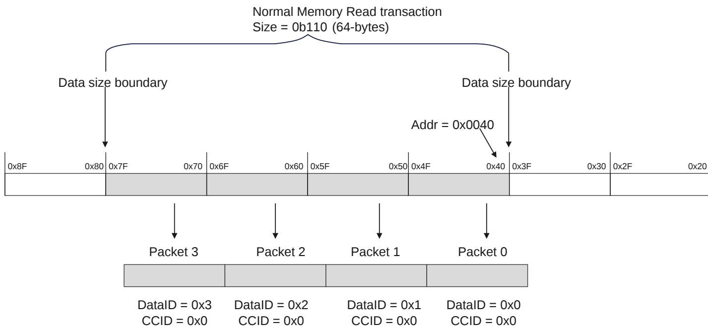
Figure B2.40: Normal memory 64-byte Read transaction from an aligned address
