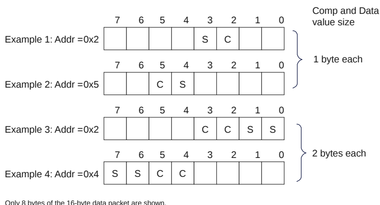
Figure B2.39: Data value packing for AtomicCompare transaction
