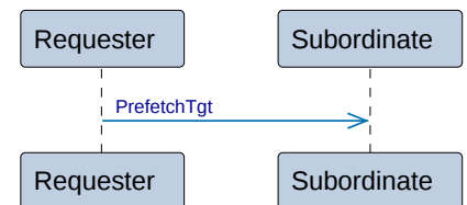
Figure B2.12: Prefetch transactions
