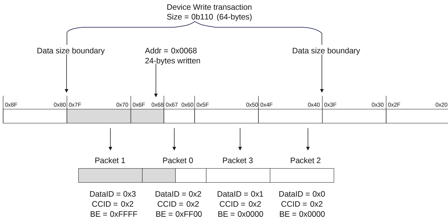
Figure B2.45: Device Write transaction to an unaligned address
