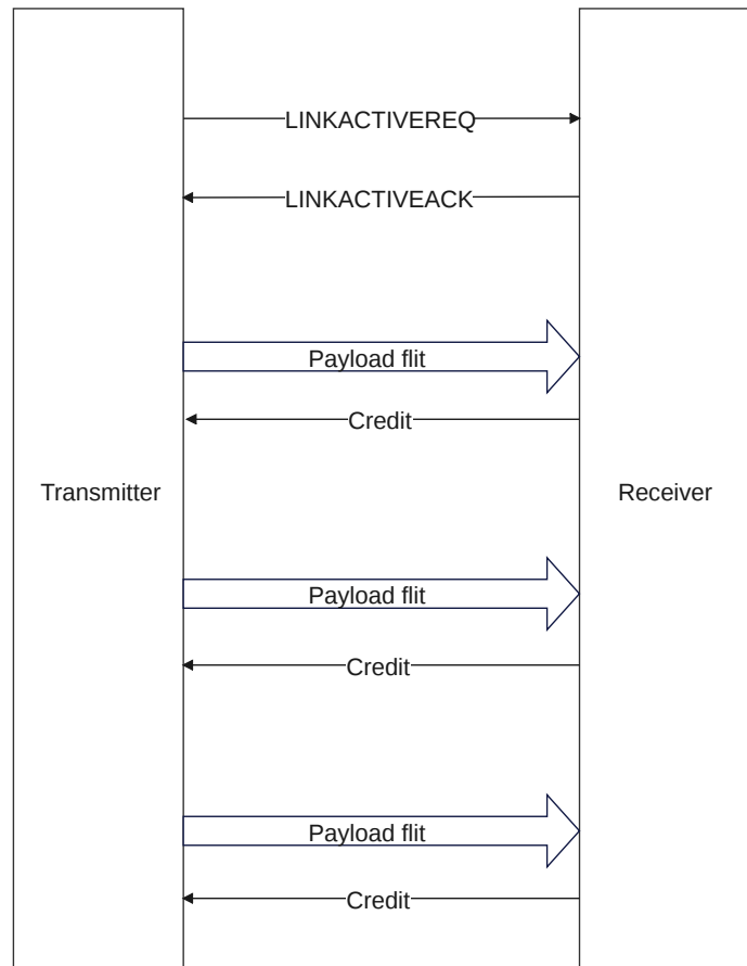
Figure B14.4: Example of a multiple channel unidirectional interface
