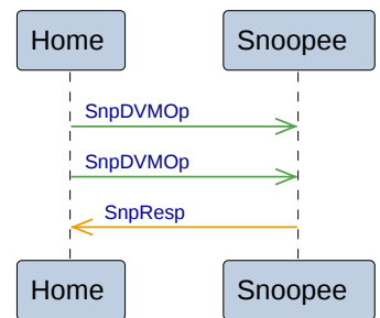
Figure B2.22: Home to Snoopee DVM transactions
