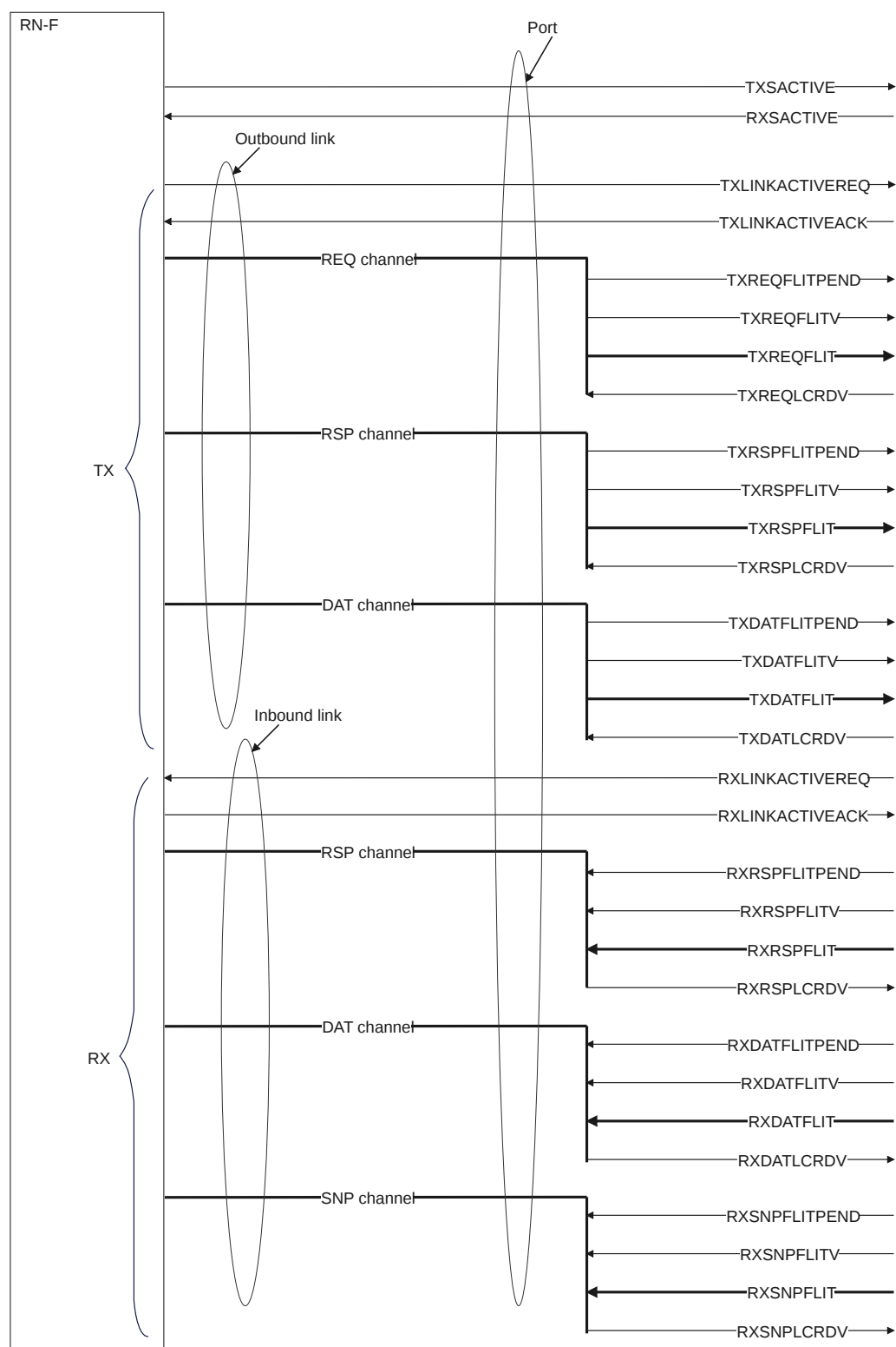
Figure B13.4: Relationship between links, channels, and ports
