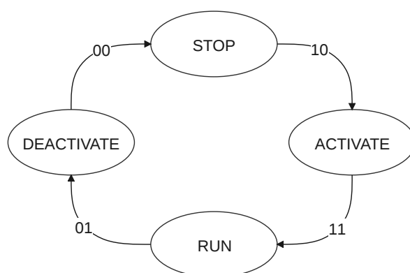
Figure B14.3: Request and Acknowledge handshake states
