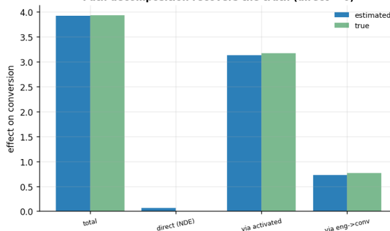
Path decomposition recovers the truth (direct \sim 0 )
