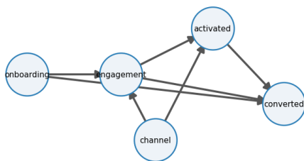
Funnel chain (direct onboarding->converted tested, \sim 0 )
