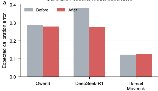
Calibration effect is model dependent
