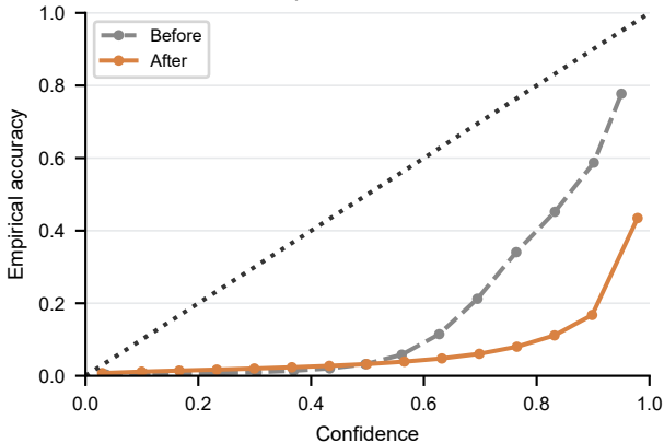
DeepSeek-R1 T=0.32
