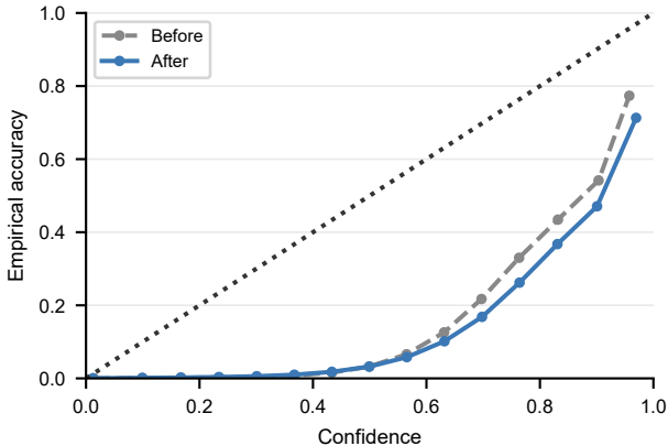
Qwen3 T=0.82
