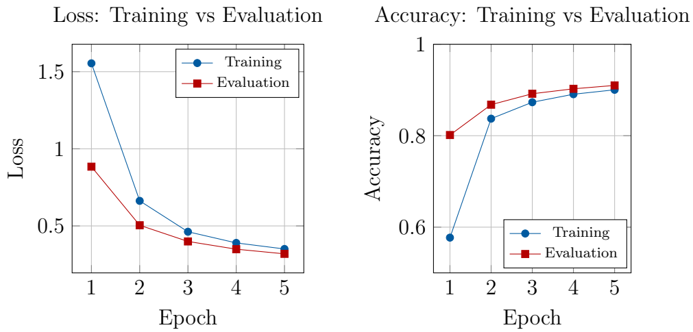
Figure 8: Perubahan loss dan accuracy selama training
