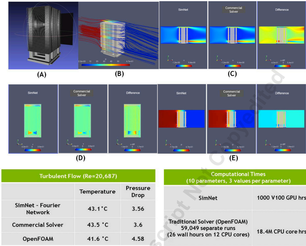
Fig. 15: Solution of conjugate heat transfer problem on a complex parameterized geometry of a heat sink for NVSwitch in DGX-A100. (A) Geometry for a heat sink with fins and heat pipes to dissipate heat from GPU, (B) Pressure color coded flow streamlines and result comparisons between SimNet and CFD commercial code for (C) U-velocity, (D) V-velocity and (E) Pressure. (Courtesy of the Nvidia team).
