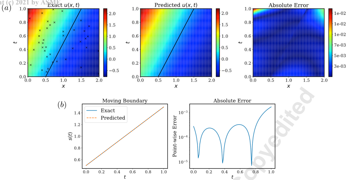
Fig. 12: Inverse two-phase Stefan problem : (a) Exact temperature solution along with training data ( \times ) versus the predicted solution. The relative L^2 error: 2.57 \cdot 10^{-3} . (b) Left : Comparison of the exact and predicted moving boundary. Right : The absolute error between the exact and the predicted free boundary for t \in [0, 1] . The L^2 error is 3.93 \cdot 10^{-4} .
