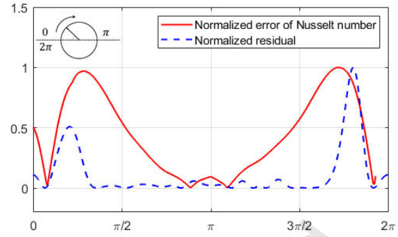
Fig. 8: Active sensor placement: the normalized error of Nusselt number and the normalized residual of the heat equation on the cylinder surface, inferred by PINN with sensor configuration Case 1 in Figure 4. We can observe the correlation between the two profiles.
