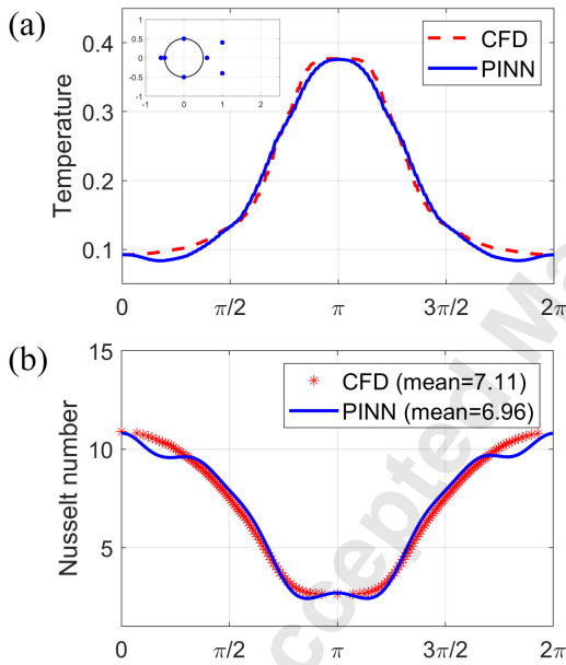
Fig. 7: Forced convection of flow past a cylinder with constant flux surface: (a) temperature and (b) Nusselt number profiles on the cylinder boundary. The sensor configuration is given at the top-left corner. With this setup, the errors of (\theta, u, v, p) inferred by PINN are 3.18%, 0.18%, 0.24% and 0.46%, respectively.
