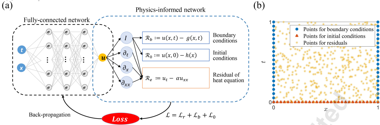
Fig. 1: Overview of physics-informed neural networks (PINNs). (a) Schematic of PINN framework. A fully-connected neural network is used to approximate the solution u(x,t) , which is then applied to construct the residual loss \mathcal{L}_r , boundary conditions loss \mathcal{L}_b and initial conditions loss \mathcal{L}_0 . The derivatives of u are computed by automatic differentiation in TensorFlow [26]. The parameters of the fully-connected network are trained by using gradient-descent methods based on the back-propagation of the loss function. (b) Schematic of point selection for PINN in the computational domain. The points with different colors correspond to different terms in the loss function. Note that the residual points for computing the residual loss can be randomly selected in the space-time domain.
