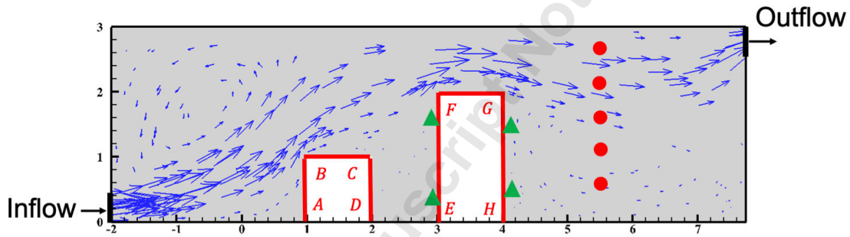
Fig. 2: Forced convection in an enclosure. The boundaries in red color are at higher temperature, and the cooling inflow enters from the left-bottom and exits at the right-top. The blue arrows show the velocity vectors. The temperature at the boundaries EF and GH are not known. The green triangles represent the temperature probes while the red circles denote the velocity probes.
