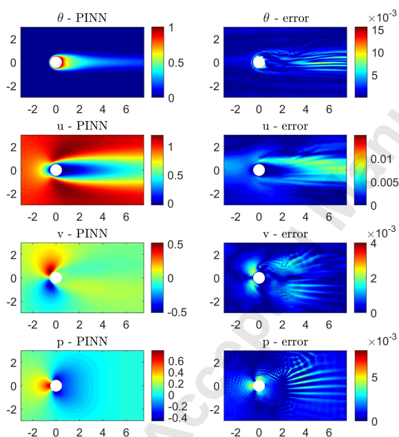
Fig. 5: Forced convection of flow past a cylinder with constant temperature surface: temperature, velocity and pressure fields inferred by PINN with sensor configuration Case 3 (left) and the point-wise absolute errors between CFD and PINN (right).
