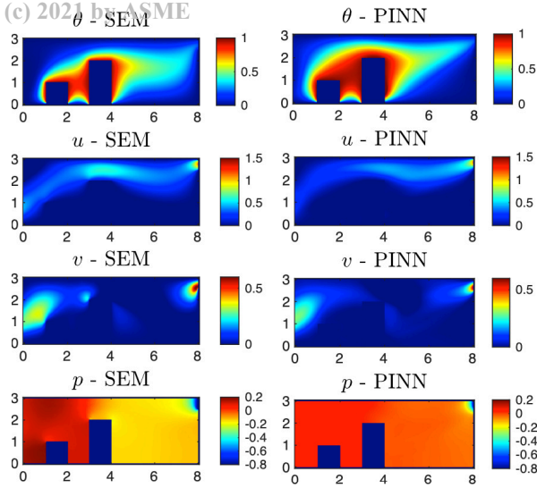
Fig. 3: Forced convection in an enclosure: comparison of \theta , u , v and p inferred by PINN and the reference simulation results by the spectral element method (SEM).
