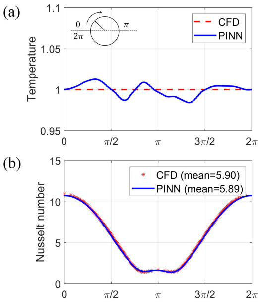
Fig. 6: Forced convection of flow past a cylinder with constant temperature surface: (a) temperature and (b) Nusselt number profiles on the cylinder boundary, inferred by PINN with sensor configuration Case 3.
