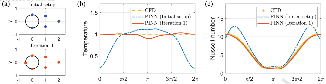
Fig. 9: Active sensor placement: (a) the sensor configurations of initial setup and after the first iteration, (b) temperature profile on the cylinder surface, (c) Nusselt number on the cylinder surface.
