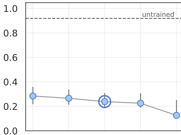
MiniLM-L12
