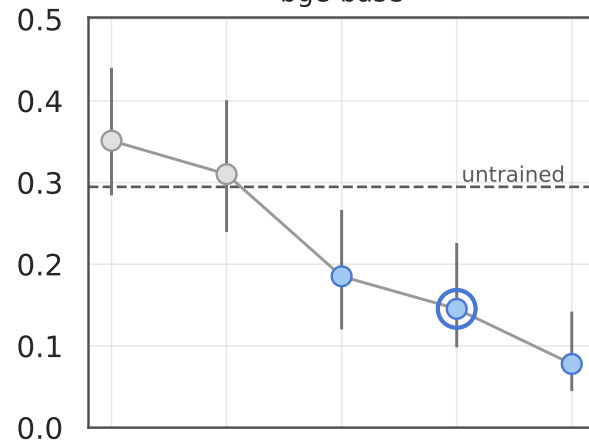
bge-base
