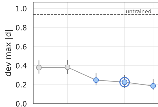
MiniLM-L6
