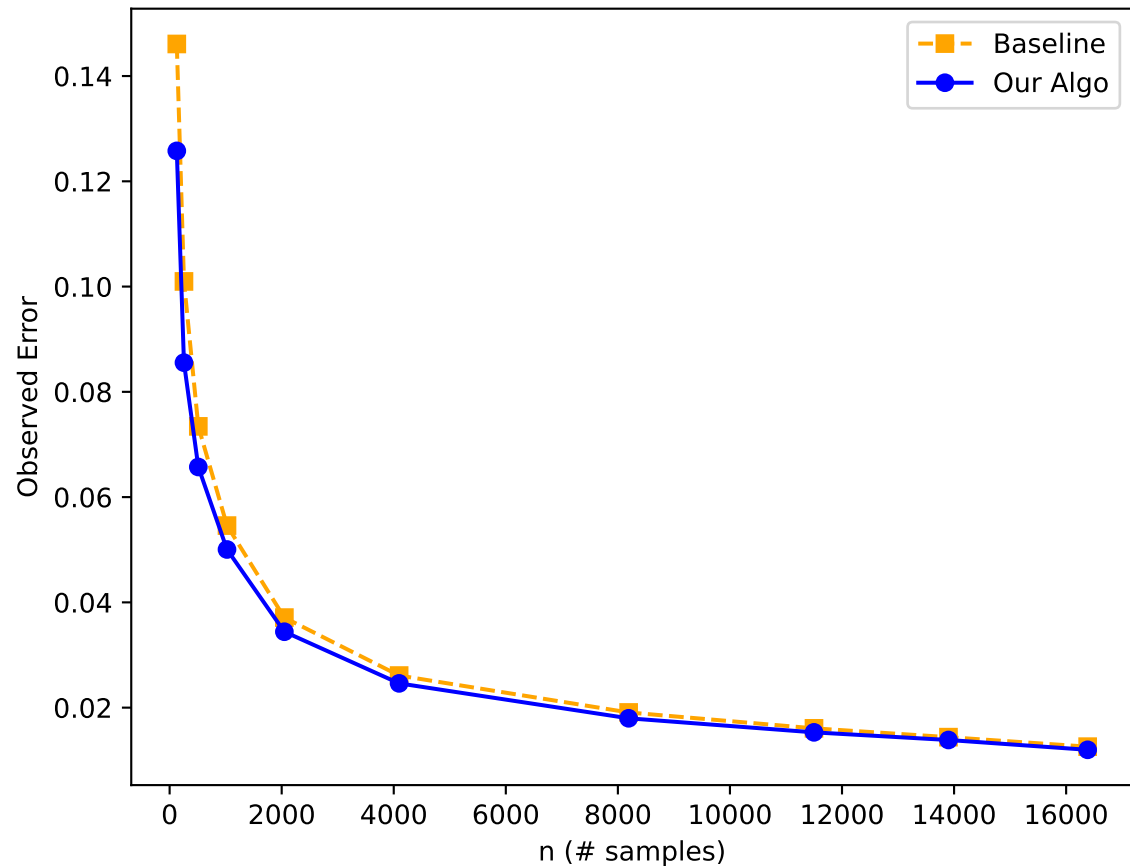
Observed Error vs n
