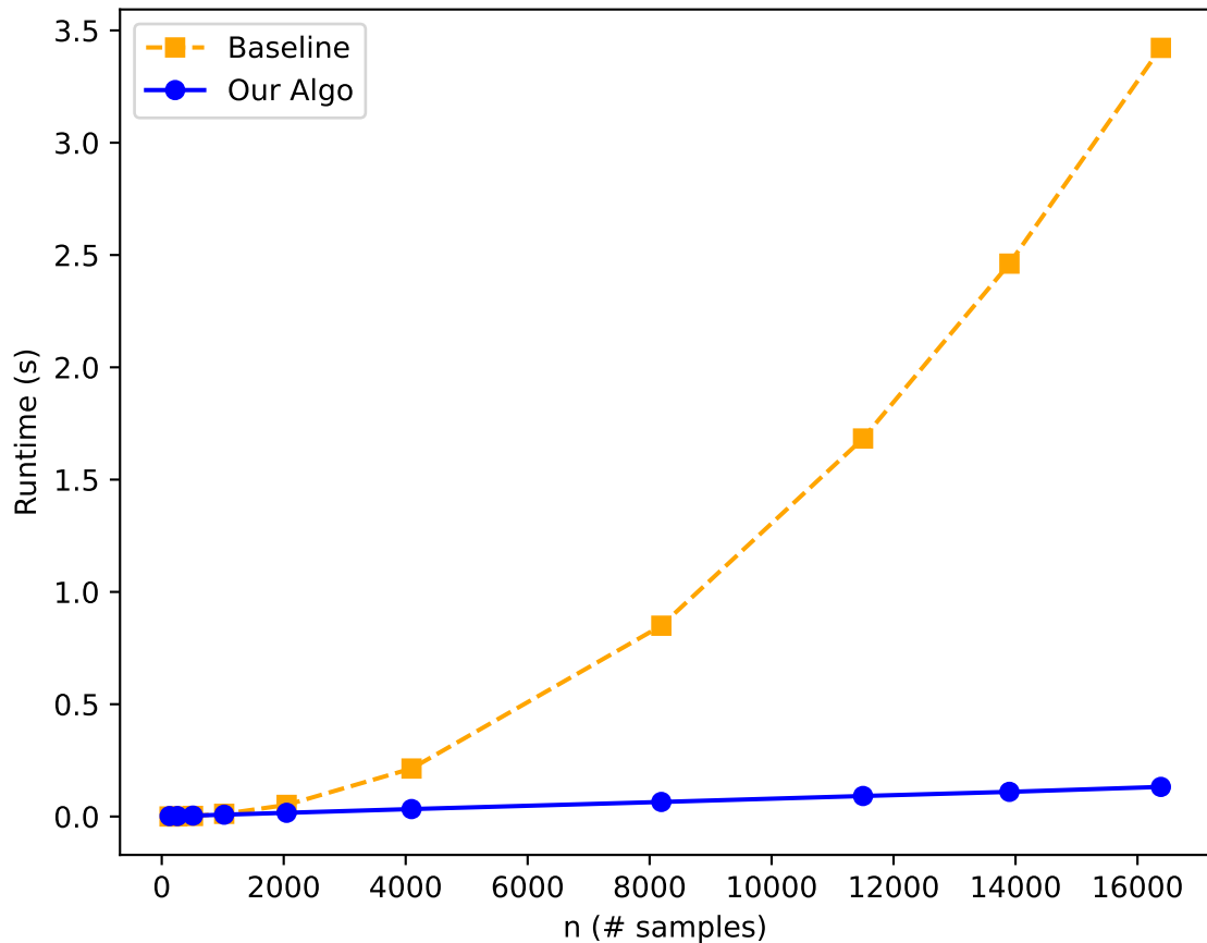
Runtime vs n
