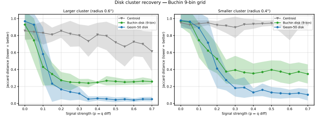
Figure 13: Circular cluster recovery on Arkansas counties: Point Jaccard distance vs. pq difference for planted disks of radius \sim 67 km (left) and \sim 44 km (right). Geom 50 (blue) recovers the correct radius at both sizes; the Buchin method (green) oversizes by \sim 20 –30% regardless of scale, giving a near-constant accuracy gap. Centroid (gray) degenerates under an unbounded disk search. Bands show \pm 1 standard deviation over 20 trials.
