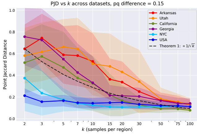
Figure 12: Point Jaccard distance as a function of k (uniformly random samples per region), at a fixed pq difference of 0.15, across all six datasets. pq = 0.15 is the transition regime where small k still fails and large k succeeds, so the diminishing-returns shape is visible on every dataset. Each curve is the mean over 20 trials with random seed 7; shaded bands show \pm 1 standard deviation. Returns diminish past k \approx 20 , motivating the abstract’s k = 20 –50 recommendation. The black dashed line overlays Theorem 5.1’s predicted asymptote d_{jac} \propto 1/\sqrt{k} , calibrated to Arkansas at the smallest sampled k ; the empirical curves track the predicted decay shape past k \approx 10 . [Foad: Per GeoInf-R1 (C2): the fine sweep over k is here, which now plots k \in \{2, 3, 5, 7, 10, 15, 20, 30, 50, 75, 100\} on all six datasets ( k = 1 is the Centroid baseline already in every main figure). The dashed black line overlays Theorem 5.1’s predicted 1/\sqrt{k} asymptote, calibrated to Arkansas at the smallest sampled k . The empirical curves track the predicted decay shape past k \approx 10 , where the (\varepsilon, \gamma) -stable regime kicks in.]
