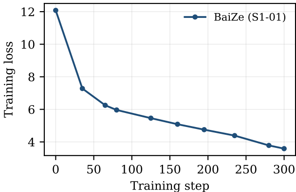
Training loss (baseline)
