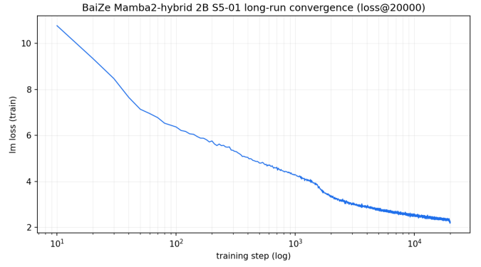
Fig. 1. Training-loss curve of the winning Mamba2-hybrid configuration over the 20000-step verification run (seed 1234); the decay tail (steps 19500–20000) anneals the loss from \sim 2.34 to 2.2054.
