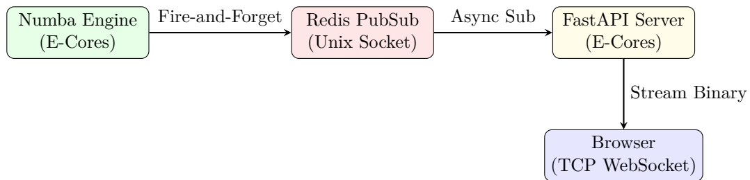
Figure 18.1: The Telemetry Network Decoupling. The matching engine is isolated from TCP network unreliability by dumping data instantly into Redis.
