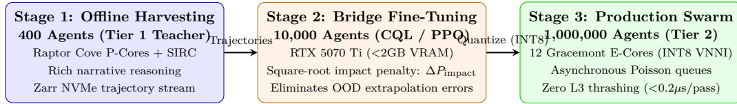
Figure 13.2: Multi-Stage Iterative Scaling Curriculum (400 → 10k → 1M agents). The three-stage pipeline bridges the microstructural distribution shift between small-scale teacher harvesting and million-agent production execution.
