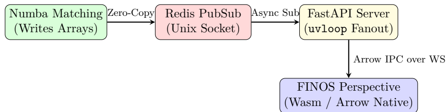
Figure 20.1: The end-to-end telemetry streaming pipeline. Decoupling matching loops from client network I/O via local Redis PubSub, WebSocket Arrow IPC streaming, and in-browser Wasm-accelerated analytics via FINOS Perspective.
