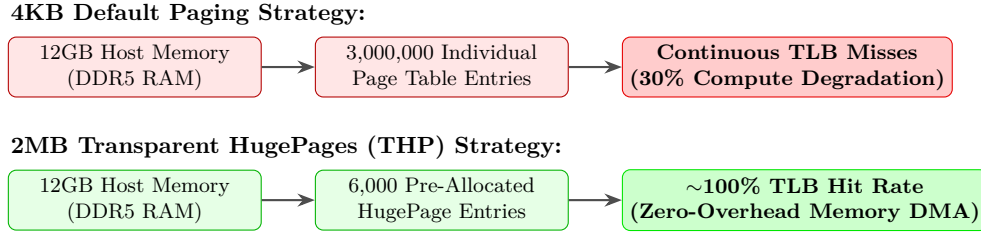
Figure C.2: Virtual address translation comparison: 4KB paging penalty versus 2MB Transparent HugePages (THP).
