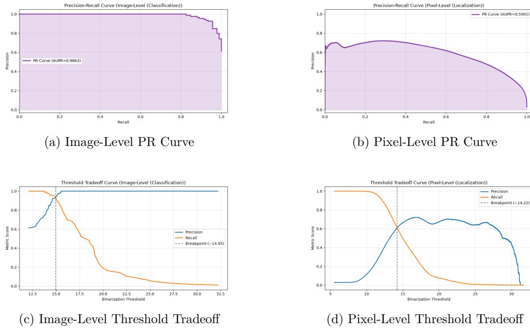
Figure 13: Evaluation curves for the cable category using PatchCore (ResNet-18). The pixel-level AUPIMO is 0.511.
