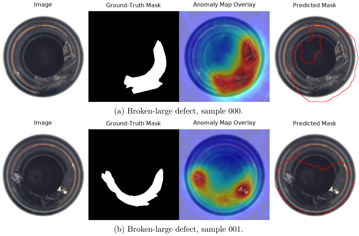
Figure 5: Four-panel qualitative results for Bottle using PatchCore (ResNet-18).
