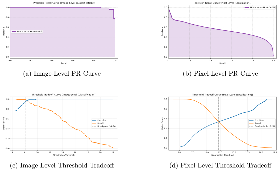
Figure 29: Evaluation curves for the carpet category using PatchCore (ResNet-18). The pixel-level AUPIMO is 0.796.
