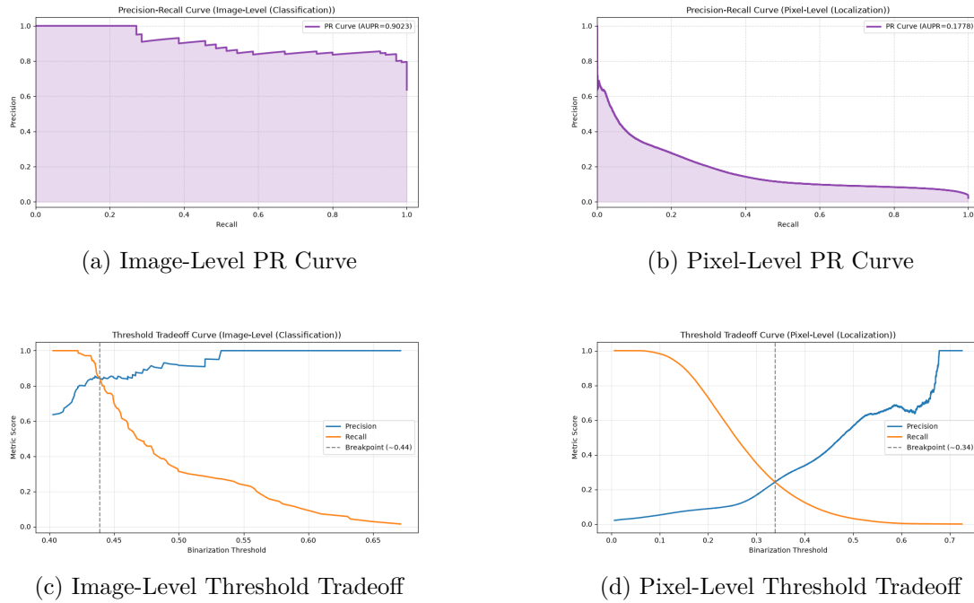
Figure 47: Evaluation curves for the hazelnut category using Keras CAE (Baseline). The pixel-level AUPIMO is 0.033.
