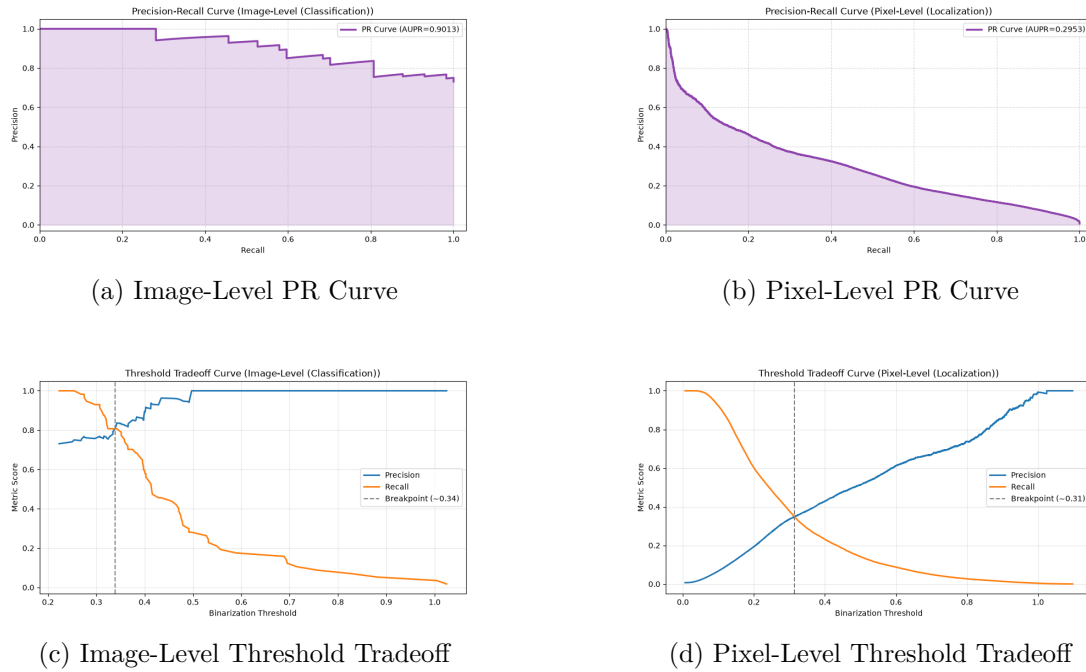
Figure 39: Evaluation curves for the grid category using Keras CAE (Baseline). The pixel-level AUPIMO is 0.077.
