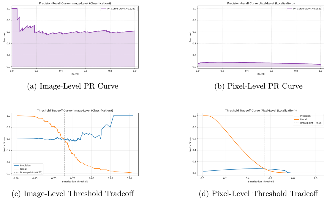
Figure 15: Evaluation curves for the cable category using Keras CAE (Baseline). The pixel-level AUPIMO is 0.000.
