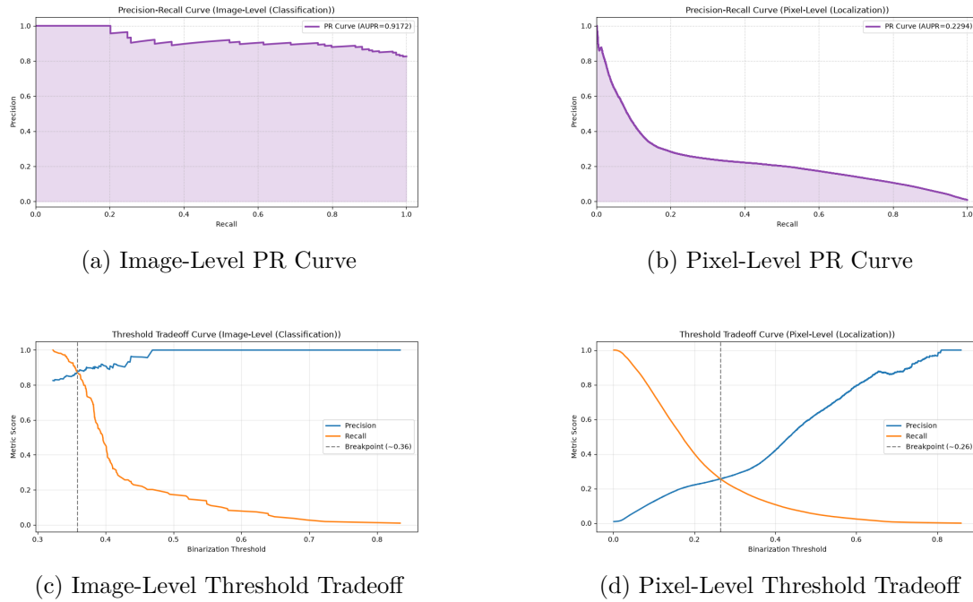
Figure 23: Evaluation curves for the capsule category using Keras CAE (Baseline). The pixel-level AUPIMO is 0.052.
