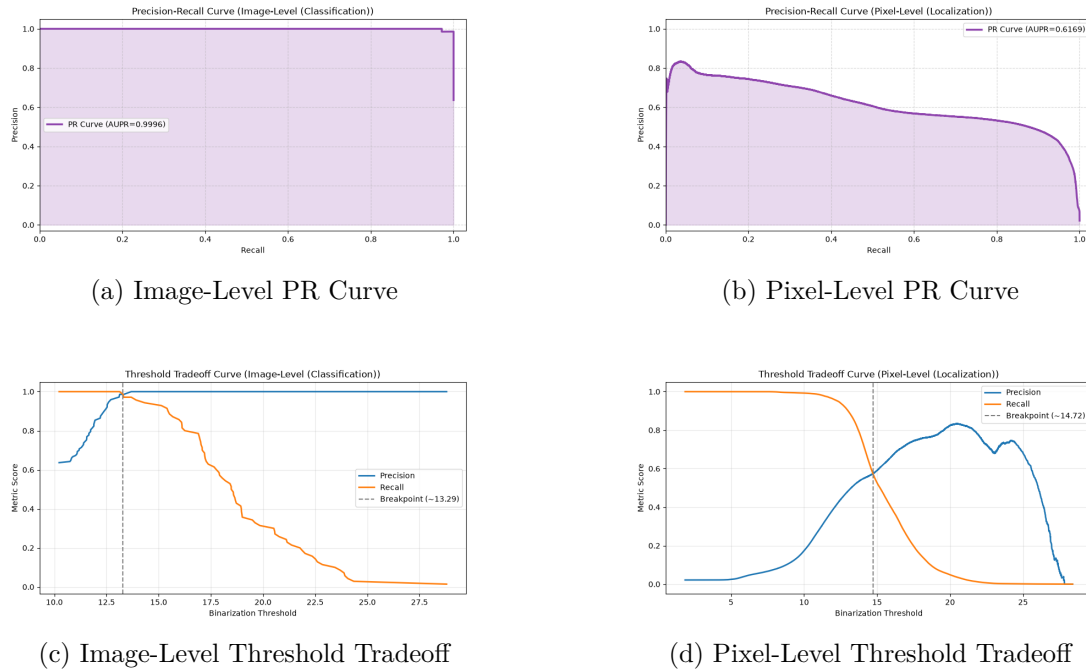
Figure 45: Evaluation curves for the hazelnut category using PatchCore (ResNet-18). The pixel-level AUPIMO is 0.863.
