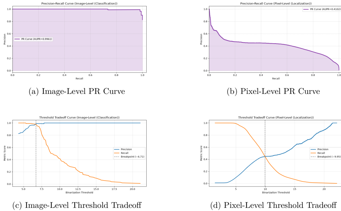
Figure 21: Evaluation curves for the capsule category using PatchCore (ResNet-18). The pixel-level AUPIMO is 0.563.
