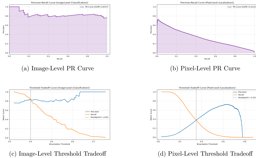
Figure 31: Evaluation curves for the carpet category using Keras CAE (Baseline). The pixel-level AUPIMO is 0.003.
