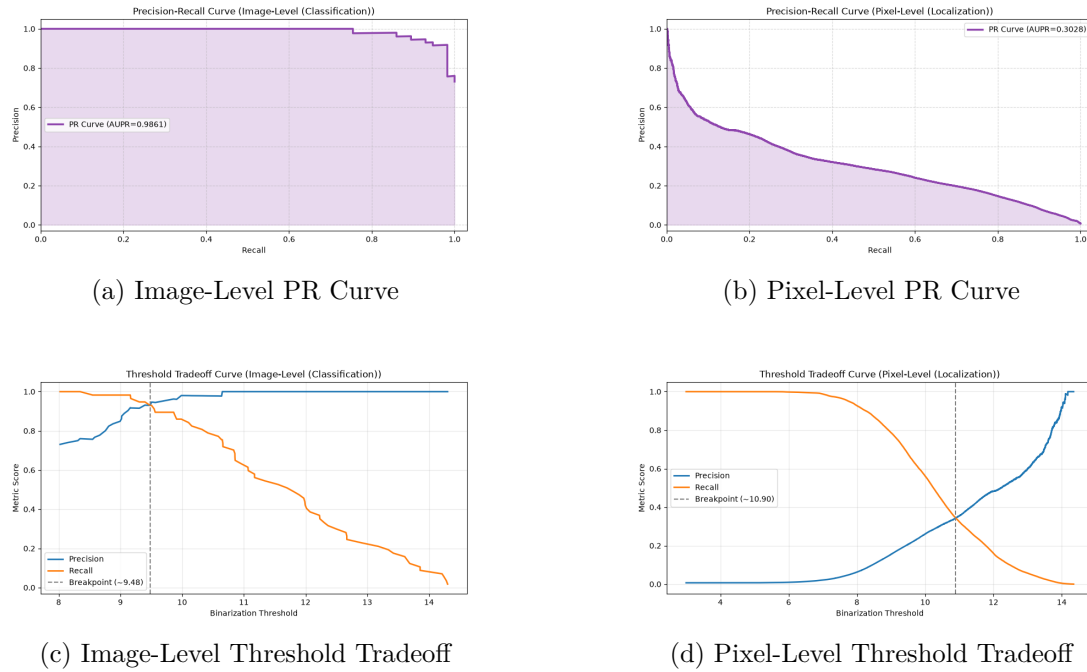
Figure 37: Evaluation curves for the grid category using PatchCore (ResNet-18). The pixel-level AUPIMO is 0.506.
