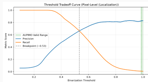
Binarization threshold curve & AUPIMO range
