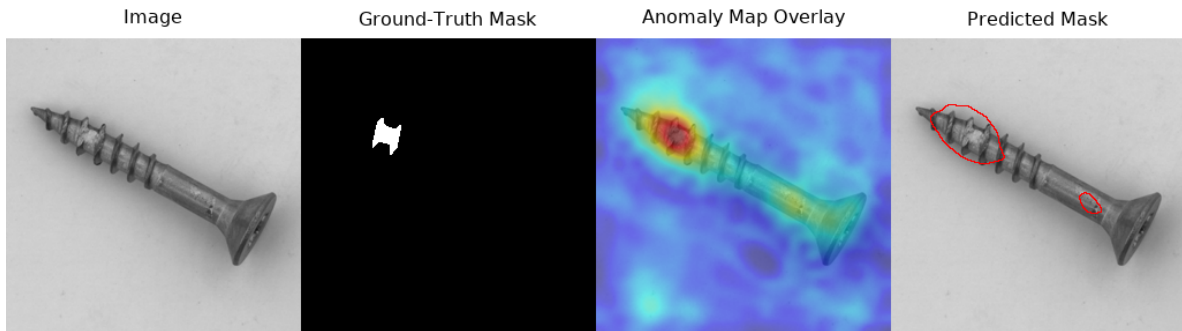
(a) Thread-top defect, sample 000.
