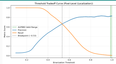
Threshold tradeoff curve & AUPIMO range
