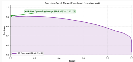
Precision-Recall curve with marked AUPIMO operating range
