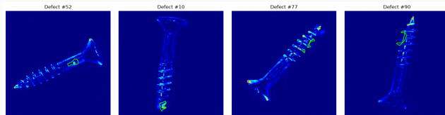
PatchCore anomaly localisations - defect contours outlining the identified anomaly regions.
