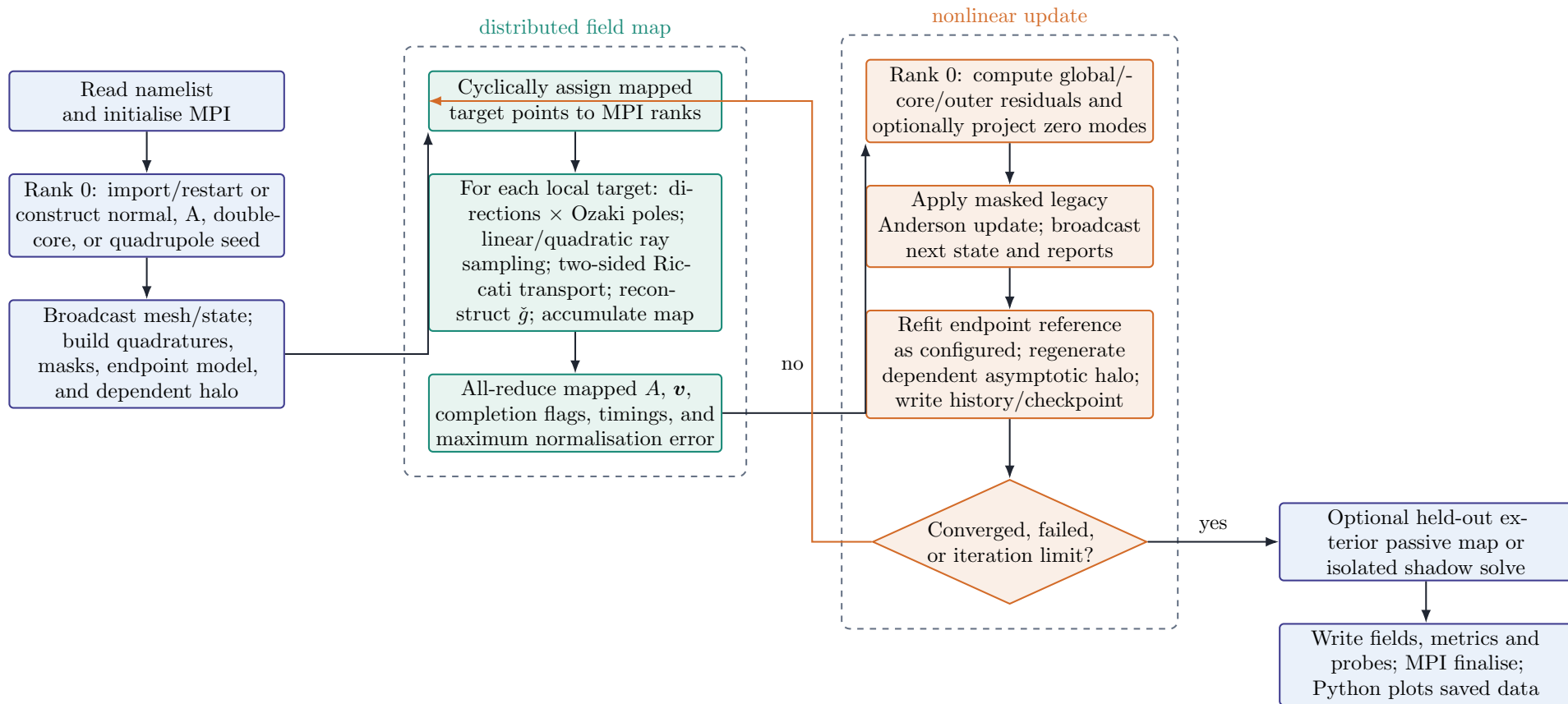
Figure 4: Implemented production algorithm. The expensive bracket is repeated for every nonlinear update. The independent exterior check is a validation stage and never feeds back into the production solution.
