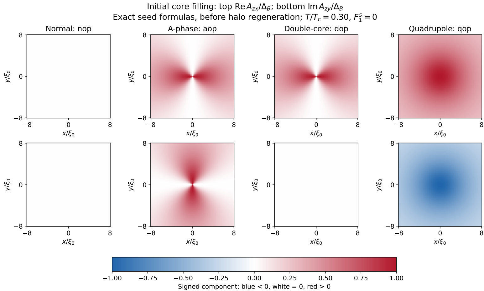
Figure 3: Two signed Cartesian components distinguish the four initializers. The common diagonal phase-wound background is omitted from the panels. All panels share the same amplitude scale; blue is negative, white is zero, red is positive. These are exact initializer formulas at t = 0.30 , F_1^s = 0 , not relaxed solutions. The \cos^2 \phi structure in the historical A and double-core seeds and the non-winding quadrupole filling are intentionally shown without smoothing or reinterpretation.
