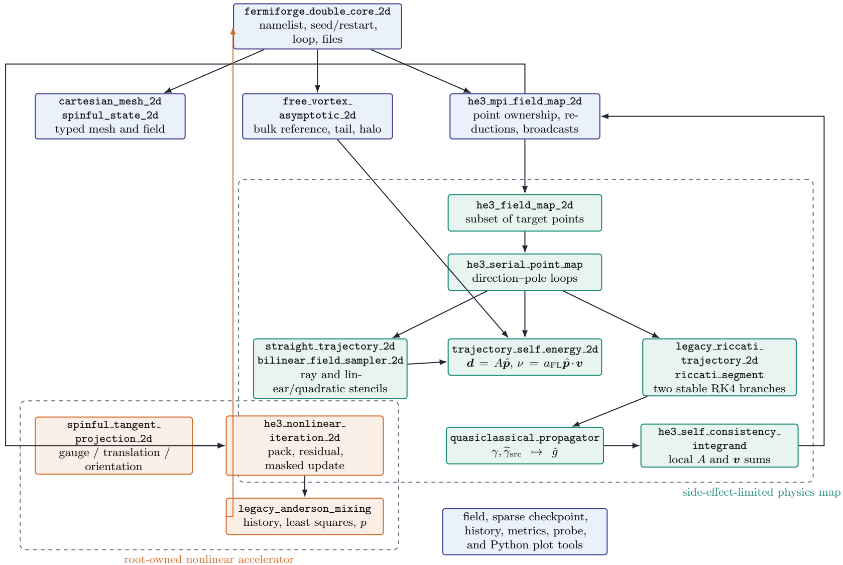
Figure 5: Principal implemented module pipeline. The reusable physics path is kept separate from MPI orchestration and from the application-level workflow.
