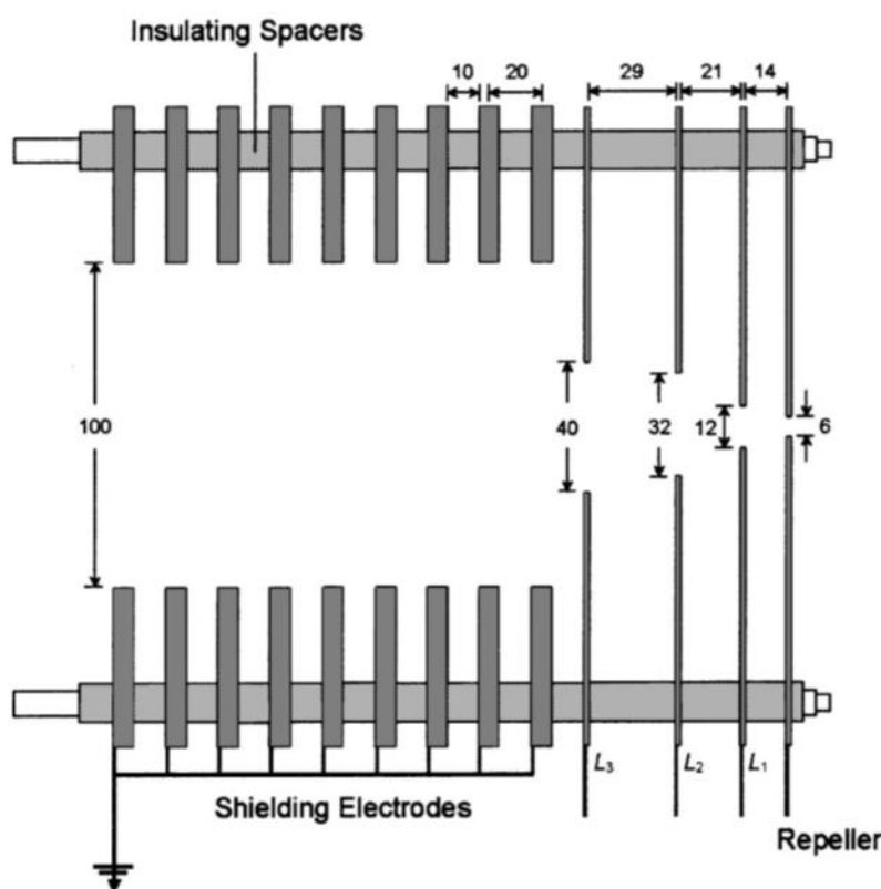
Fig. 2.3 Schematic of the ion lens assembly containing the four electrodes repeller, extractor ( L_1 ), focusing lens 1 ( L_2 ), and focusing lens 2 ( L_3 ). Units are in mm. Adapted with permission from D. Townsend et al, Rev. Sci. Instrum. , 74(4), 2530–2539 (2003) © AIP.
