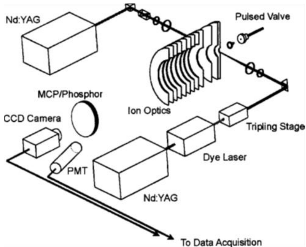
Fig. 2.4 Schematic of the experimental setup with a cut-through of the ion optics assembly. Adapted with permission from D. Townsend et al, Rev. Sci. Instrum. , 74(4), 2530–2539 (2003) © AIP.
