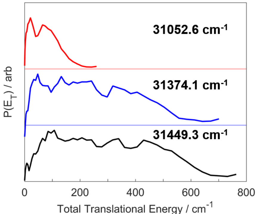
Fig. 5.6 D atom translational energy distributions of three selected images displayed in Figure 5.4.
