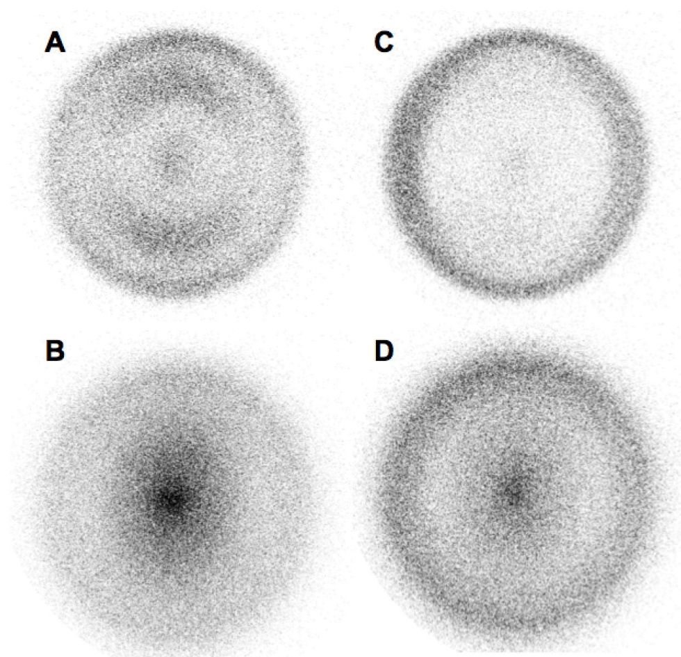
Fig. 4.1 DC slice images of 1-color UV Cl (A), 2-color Cl (B), 1-color UV Cl* (C), and 2-color Cl* (D) from photodissociation of propargyl chloride. Laser polarization axis is vertical in the plane of the figure.
