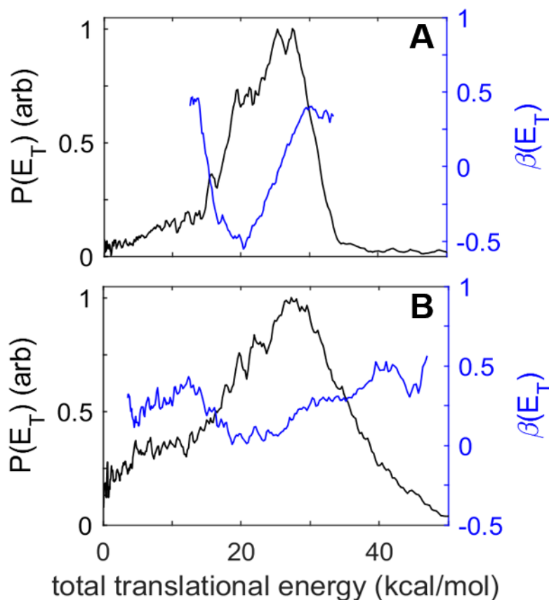
Fig. 4.4 Translational energy distributions (black) and anisotropy parameter \beta (blue) of Cl* from 1-color UV (A) and 2-color (B) experimental configurations of propargyl chloride photodissociation.
