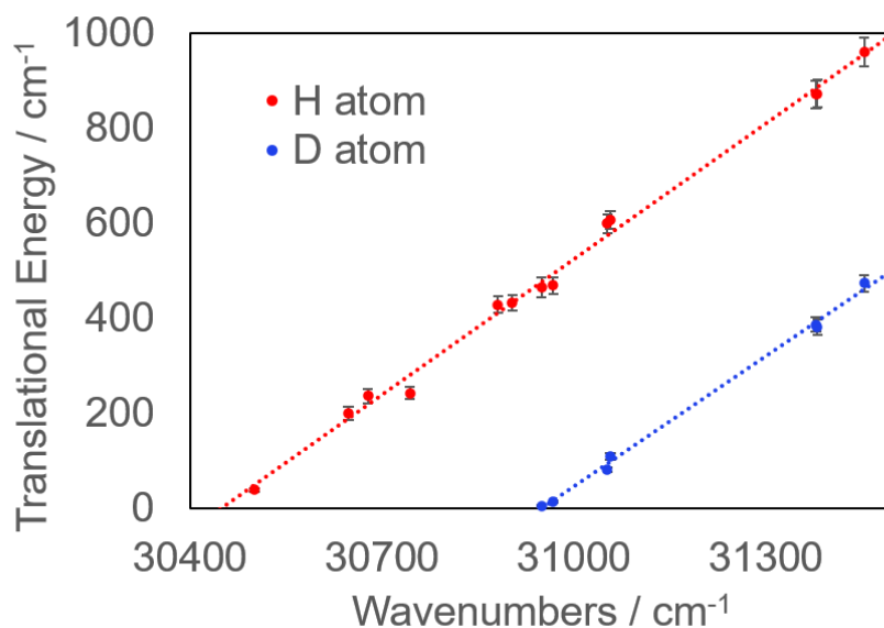
Fig. 5.5 Translational energy plotted against upper state energy for H atom (red) and D atom (blue) fragments.
