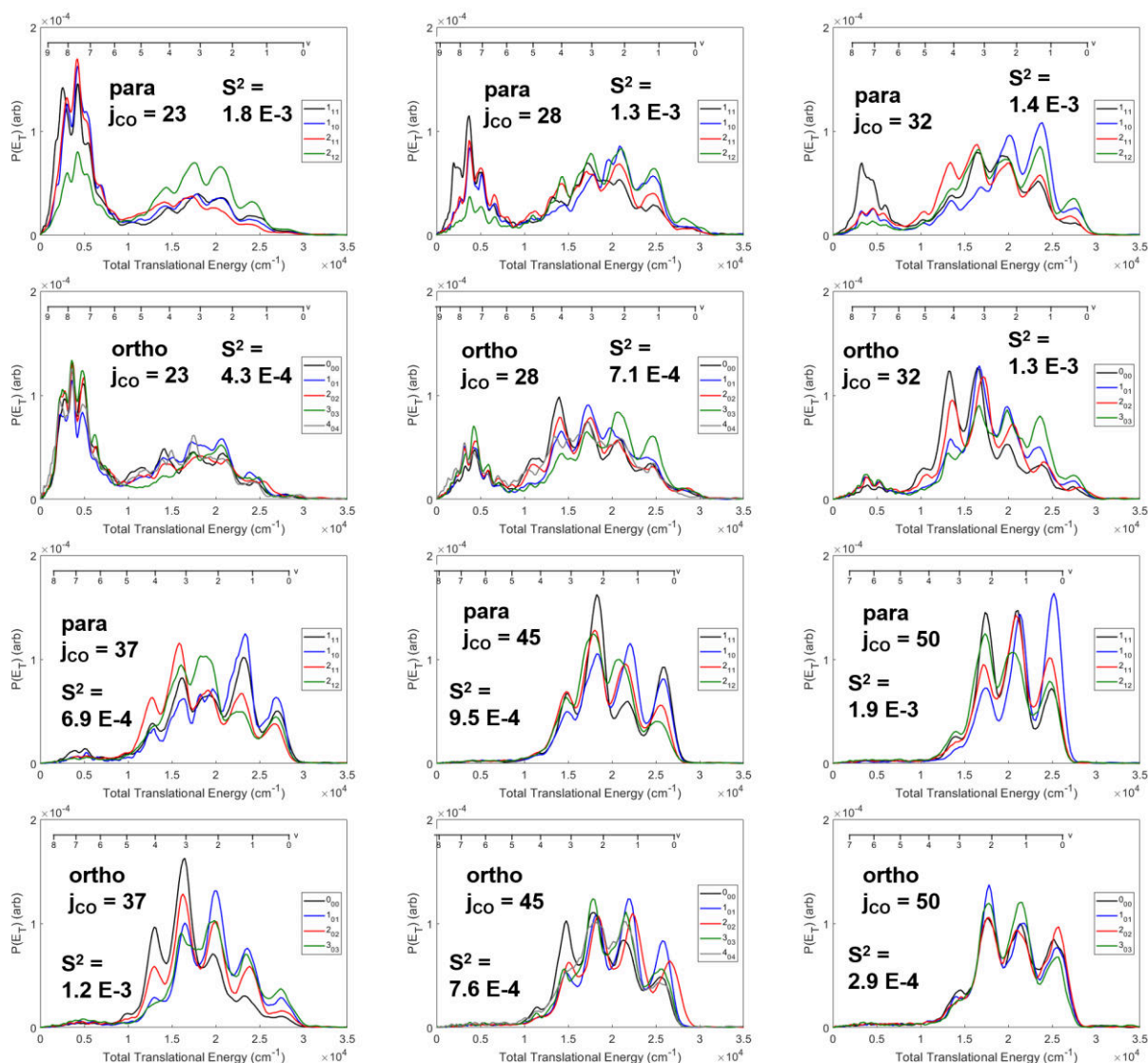
Fig. 6.4 Total translational energy distributions of a series j_{\text{CO}} images for a series of ortho and para excitations of 2^{143} .
