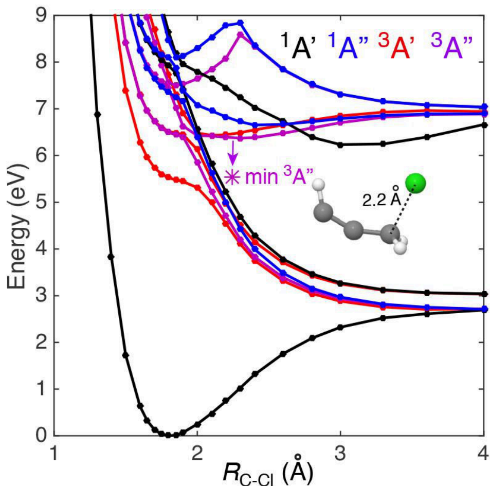
Fig. 3.8 Potential energy cuts along the \text{RC-Cl} coordinate leading to the \text{C}_3\text{H}_3 + \text{Cl} and \text{C}_3\text{H}_3^* + \text{Cl} asymptotes. The level of theory is SA12- CASSCF(10/11)/cc-pVTZ and the geometry is relaxed on the ground state by optimization at the MP2/cc-pVTZ level. The color code for state symmetry and multiplicity is the same as in Fig. 5. The molecular structure corresponds to a minimum on the 2^3A'' state, which correlates to the \text{C}_3\text{H}_3^* + \text{Cl} asymptote and could play a role as an intermediate before the dissociation occurs towards the ground state.
