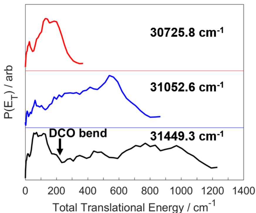
Fig. 5.7 H atom translational energy distributions of three selected images displayed in Figure 5.4.
