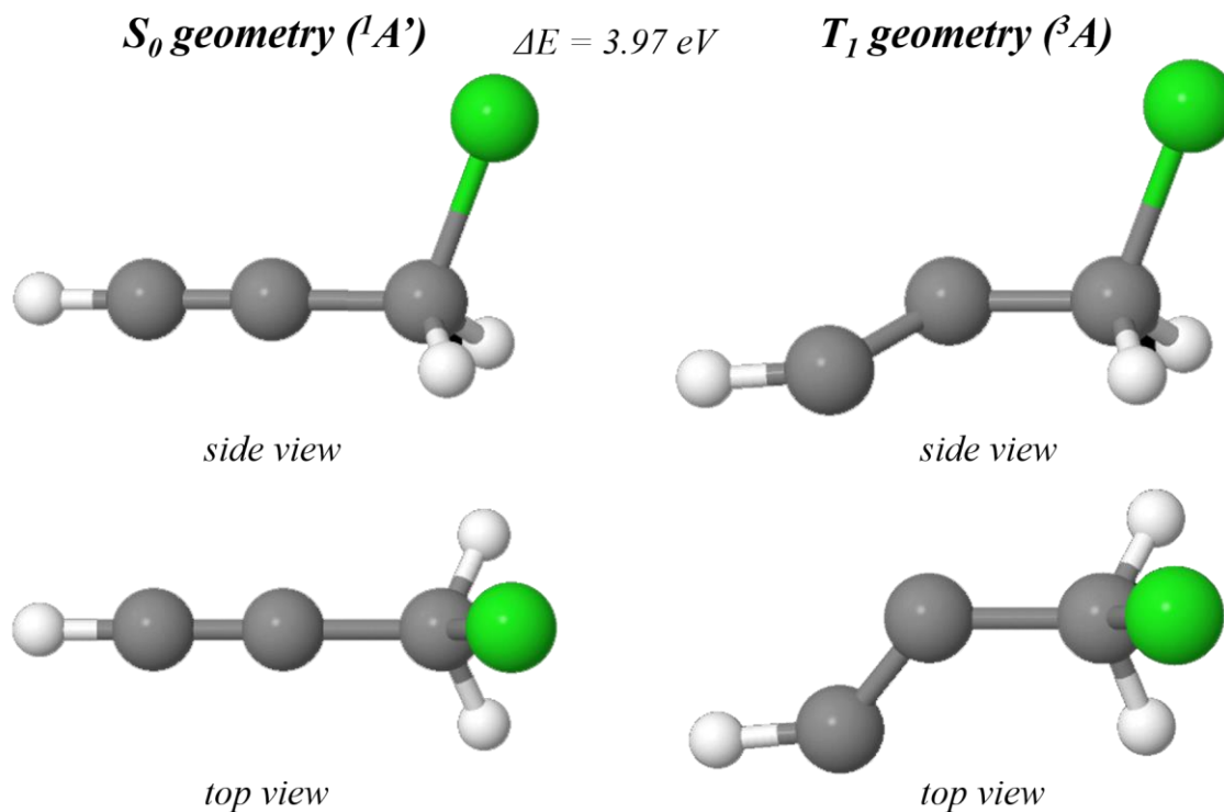
Fig. 3.1 Structures of the ^1A' and ^3A minima optimized at the CCSD(T) level, along with singlet–triplet separation energy, \Delta E , including ZPE correction.
