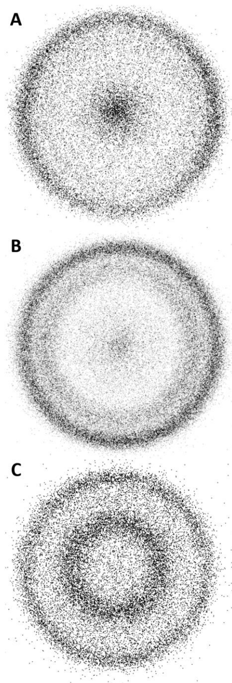
Fig. 3.4 DC slice images of Cl (A) Cl* (B) and C 3 H 3 (C) from photodissociation of propargyl chloride near 212 nm. Laser polarization axis is vertical.
