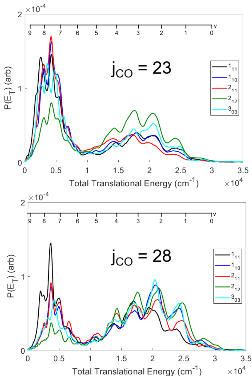
Fig. 6.13 Total translational energy distributions for j_{\text{CO}} = 23 and 28 for excitations near the identified resonance.
