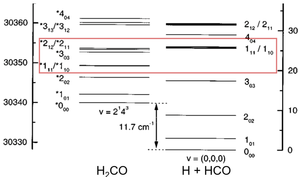
Fig. 6.11 Energy ladder of \text{H}_2\text{CO} (left) and \text{H} + \text{HCO} (right) rotational states. The states involved in a resonance are indicated by the red box. Adapted with permission from A.C. Terentis et al, J. Chem. Phys. , 108 (8), 3187–3198 (1998) © AIP.
