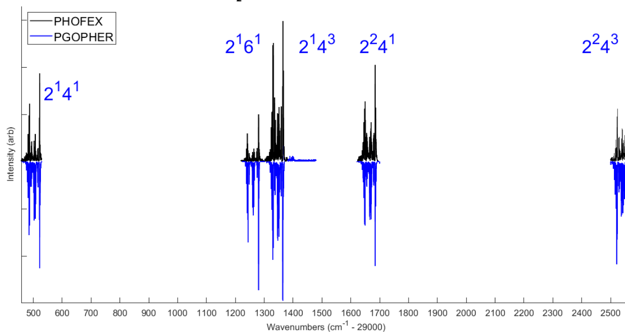
H 2 CO PHOFEX spectrum, J=44 CO
