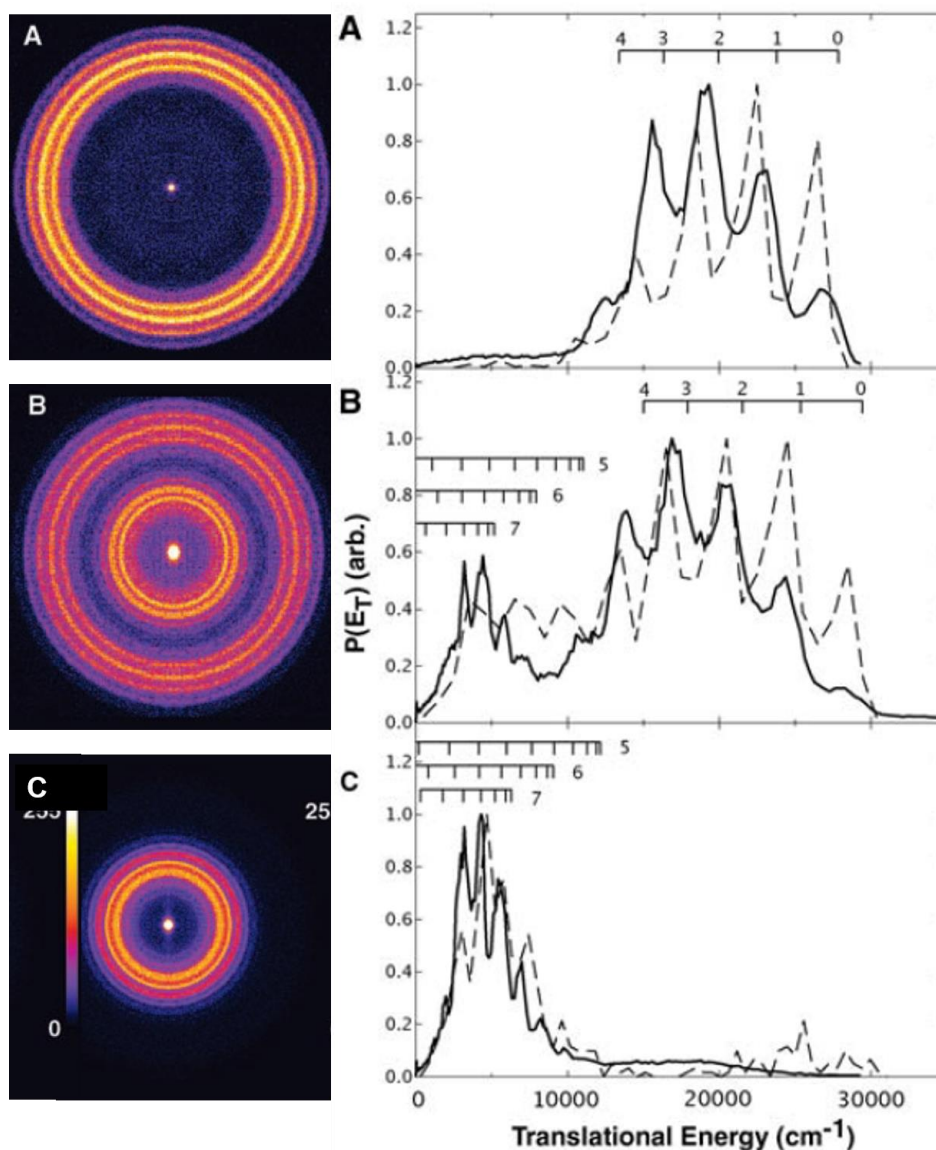
Fig. 1.2 Left. Ion images of j_{CO} = 40 (A), j_{CO} = 28 (B), and j_{CO} = 15 (C). Right. Solid lines are experimental translational energy distributions of the corresponding images and dashed lines are determined by quasi-classical trajectories. Combs indicate the H_2 vibrational state. Adapted with permission from D. Townsend et al, Science , 306, 1158–1161 (2004) © AAAS.
