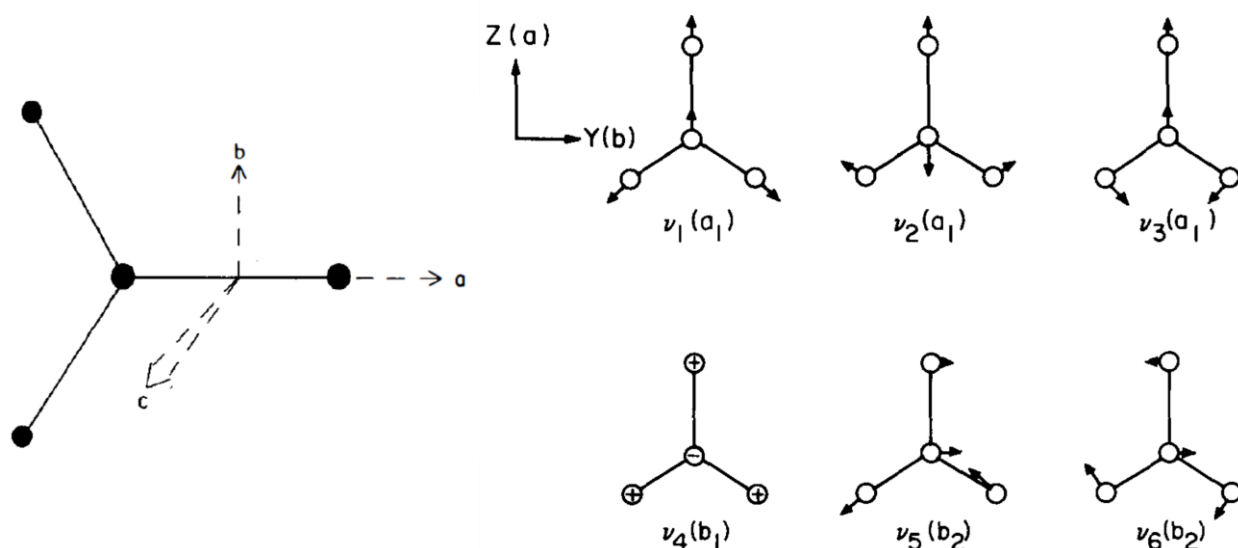
Fig. 5.2 Left. Inertial axis designations. Right. Normal modes of vibration and symmetry species. Adapted with permission from D.J. Clouthier et al, Ann. Rev. Phys. Chem. , 34, 31–58 (1983) © Annual Reviews and D.E. Reisner et al, J. Chem. Phys. , 80(12), 5968–5978 (1983) © AIP.
