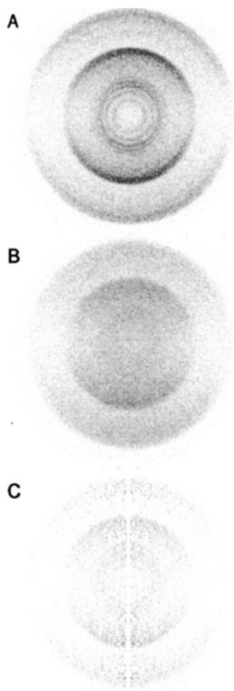
Fig. 2.2 Images of O(^3P_2) that are DC sliced (A), unsliced (B), and unsliced and reconstructed. Adapted with permission from D. Townsend et al, Rev. Sci. Instrum. , 74(4), 2530–2539 (2003) © AIP.
