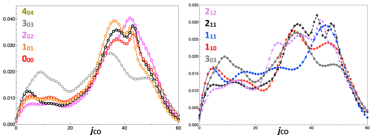
Fig. 6.2 Rotational distributions for CO ( v = 0 ) following excitation of a range of parent \text{H}_2\text{CO} rotational levels on the 2^1 4^3 band. All have been normalized to the same total population.
