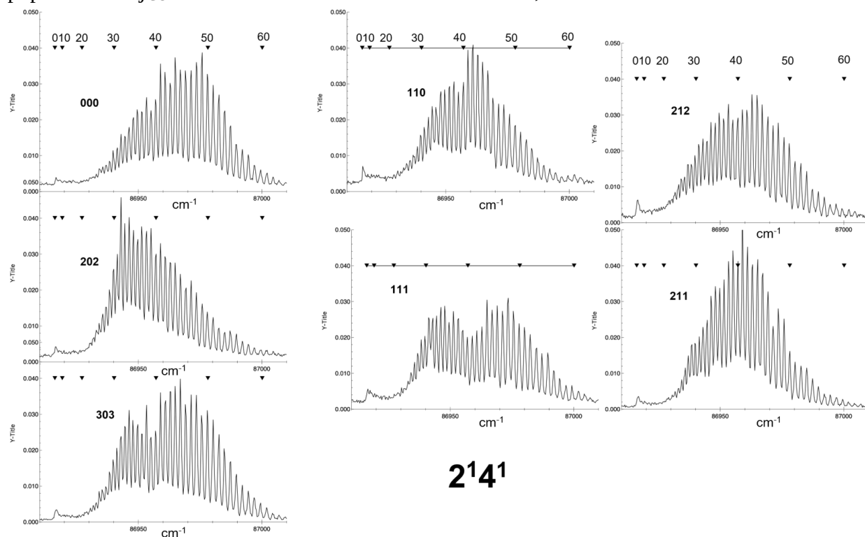
Fig. 6.6 Raw CO REMPI spectra for several ortho and para excitations on the 2^14^1 band.
