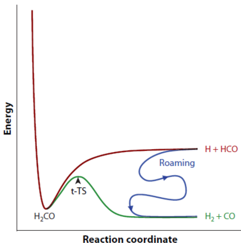
Fig. 1.1 Schematic illustration of S_0 dissociation pathways of formaldehyde. Adapted with permission from A.G. Suits, Ann. Rev. Phys. Chem. , 71, 77–100 (2020) © Annual Reviews.
