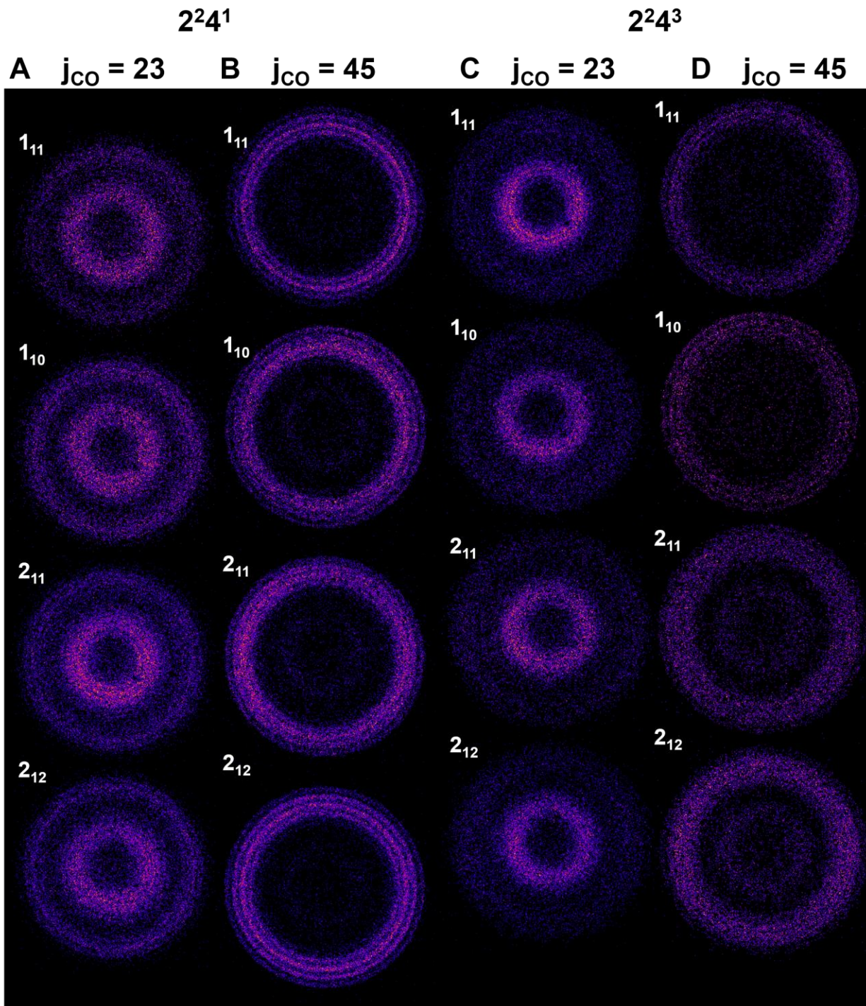
Fig. 6.7 DC slice images of j_{\text{CO}} = 23 dissociated from 2^2 4^1 (A), j_{\text{CO}} = 45 dissociated from 2^2 4^1 (B), j_{\text{CO}} = 23 dissociated from 2^2 4^3 (C), j_{\text{CO}} = 45 dissociated from 2^2 4^3 (D).
