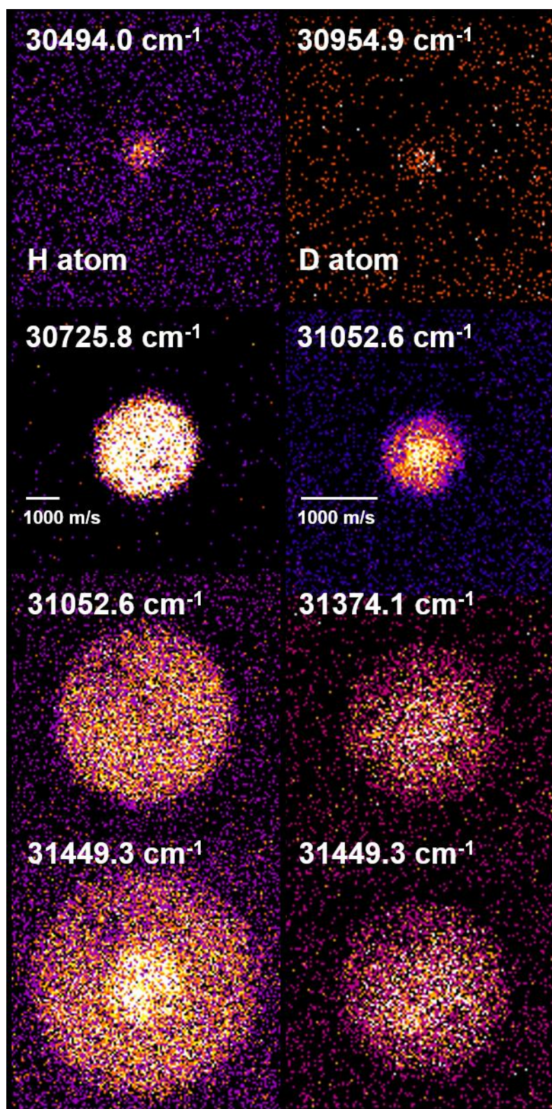
Fig. 5.4 Selected images of H atom (left column) and D atom fragments (right column) from excitation on different rovibrational lines of HDCO.
