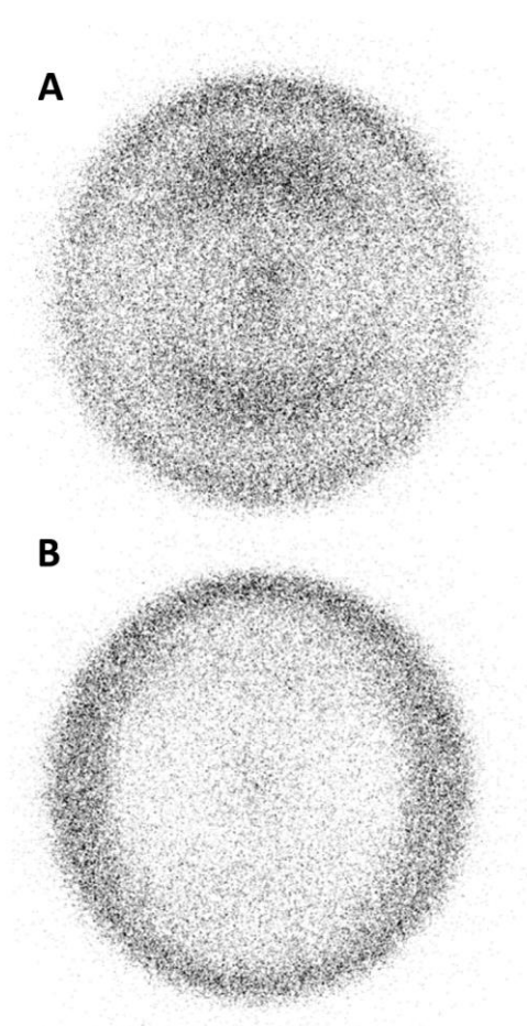
Fig. 3.2 DC slice images of Cl (A) and Cl* (B) from photodissociation of propargyl chloride near 236 nm. Laser polarization axis is vertical.
