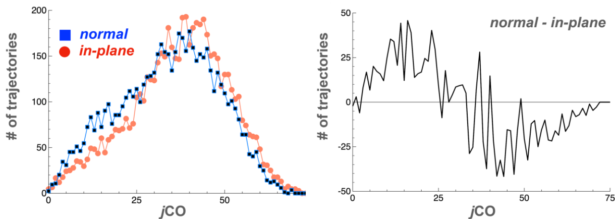
Fig. 6.14 In-plane restricted (red) vs. normal (blue) trajectory results.
