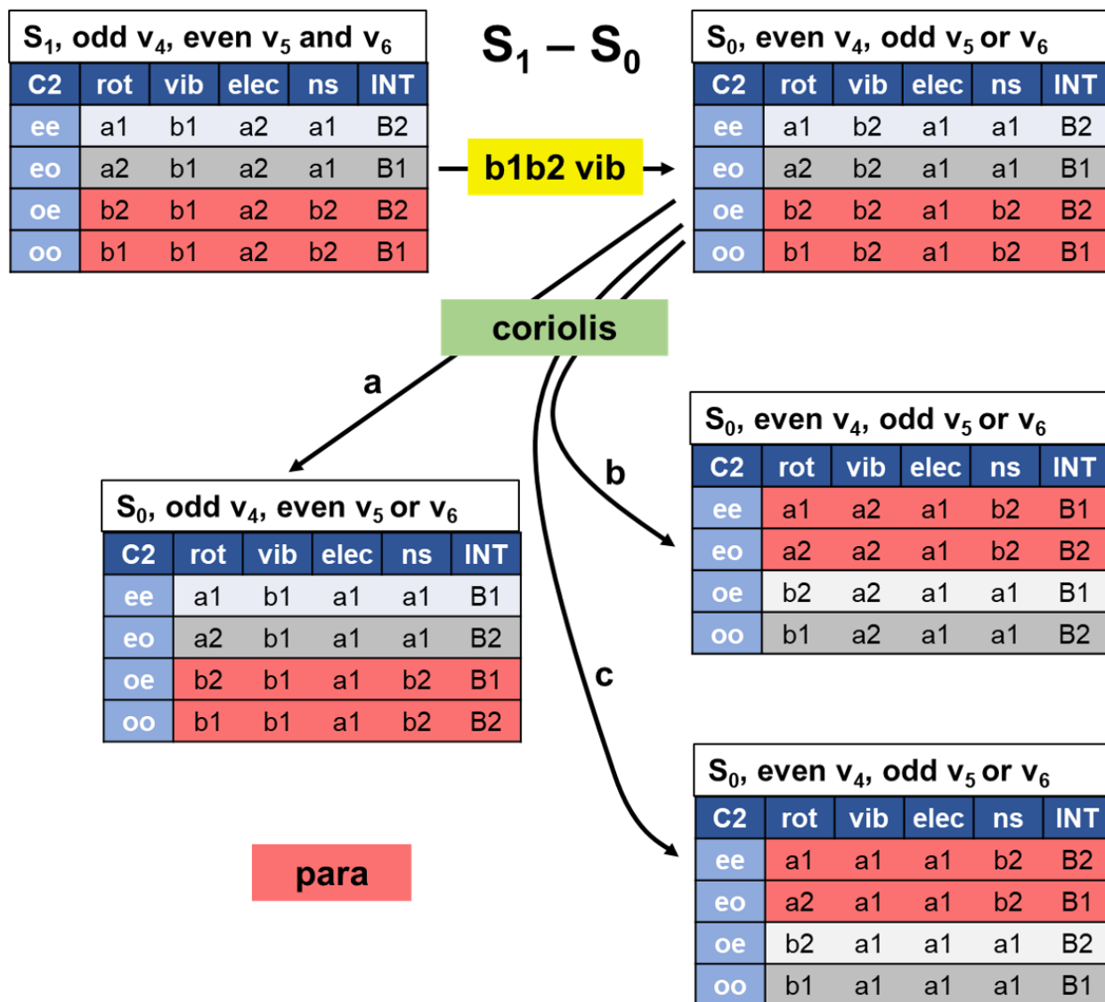
Fig. 6.10 Symmetry coupling “blocks” describing how an initially prepared state on S_1 couples to S_0 .
