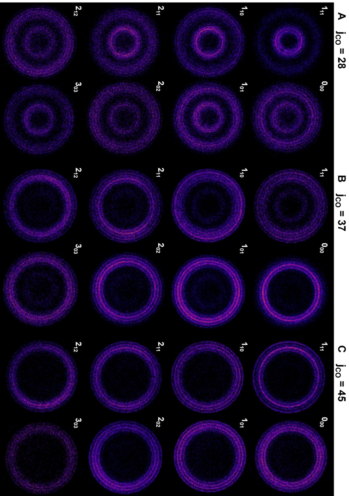
Fig. 6.3 DC slice images of j_{co} = 28 (A), j_{co} = 37 (B) and j_{co} = 45 (B) for a series of ortho and para excitations of 2^{14}_3 .
