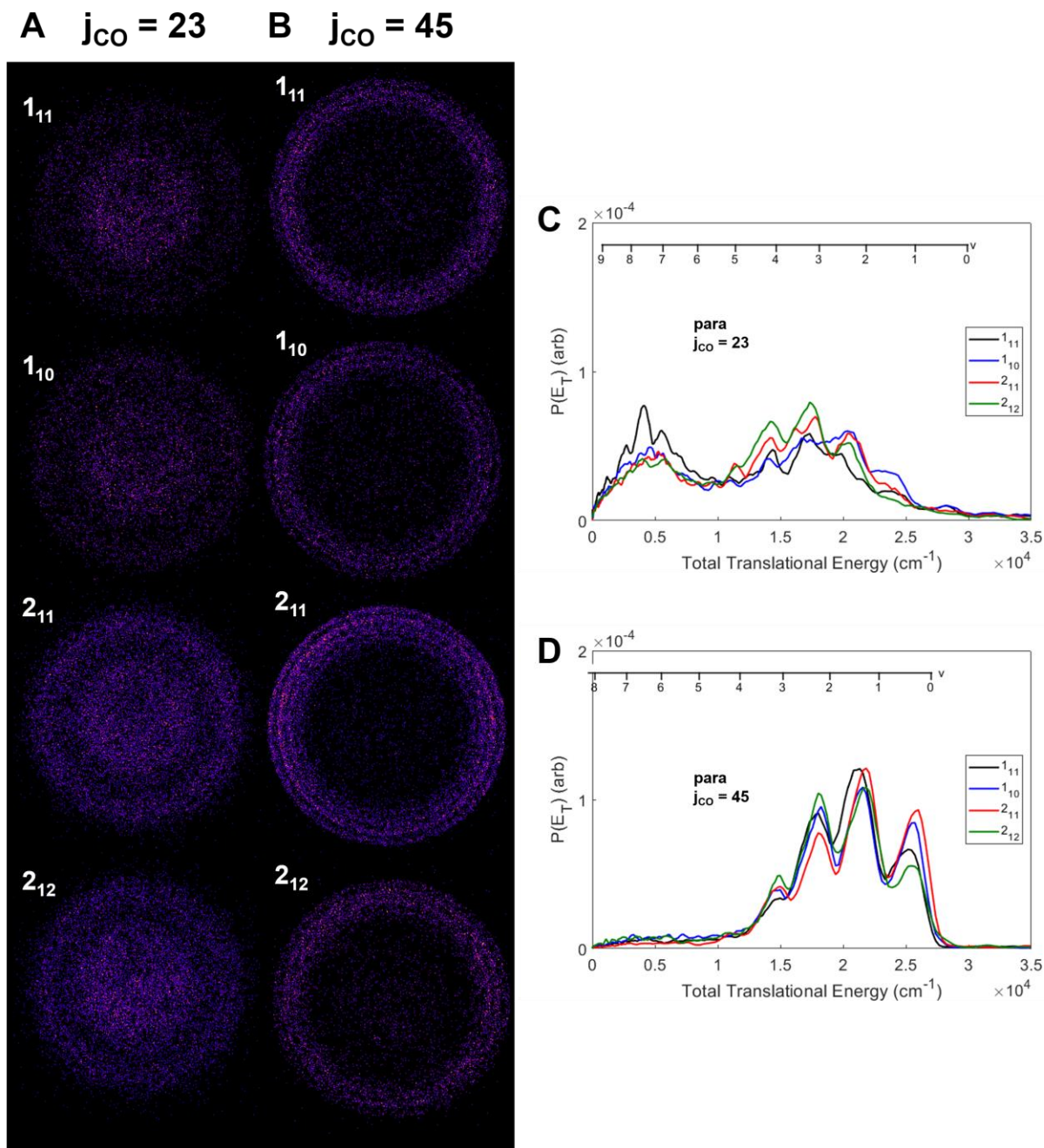
Fig. 6.5 DC slice images of a series of 2^1 6^1 para excitations of j_{\text{CO}} = 23 (A) and j_{\text{CO}} = 45 (B). Associated total translational energy distributions of j_{\text{CO}} = 23 (C) and j_{\text{CO}} = 45 (D).
