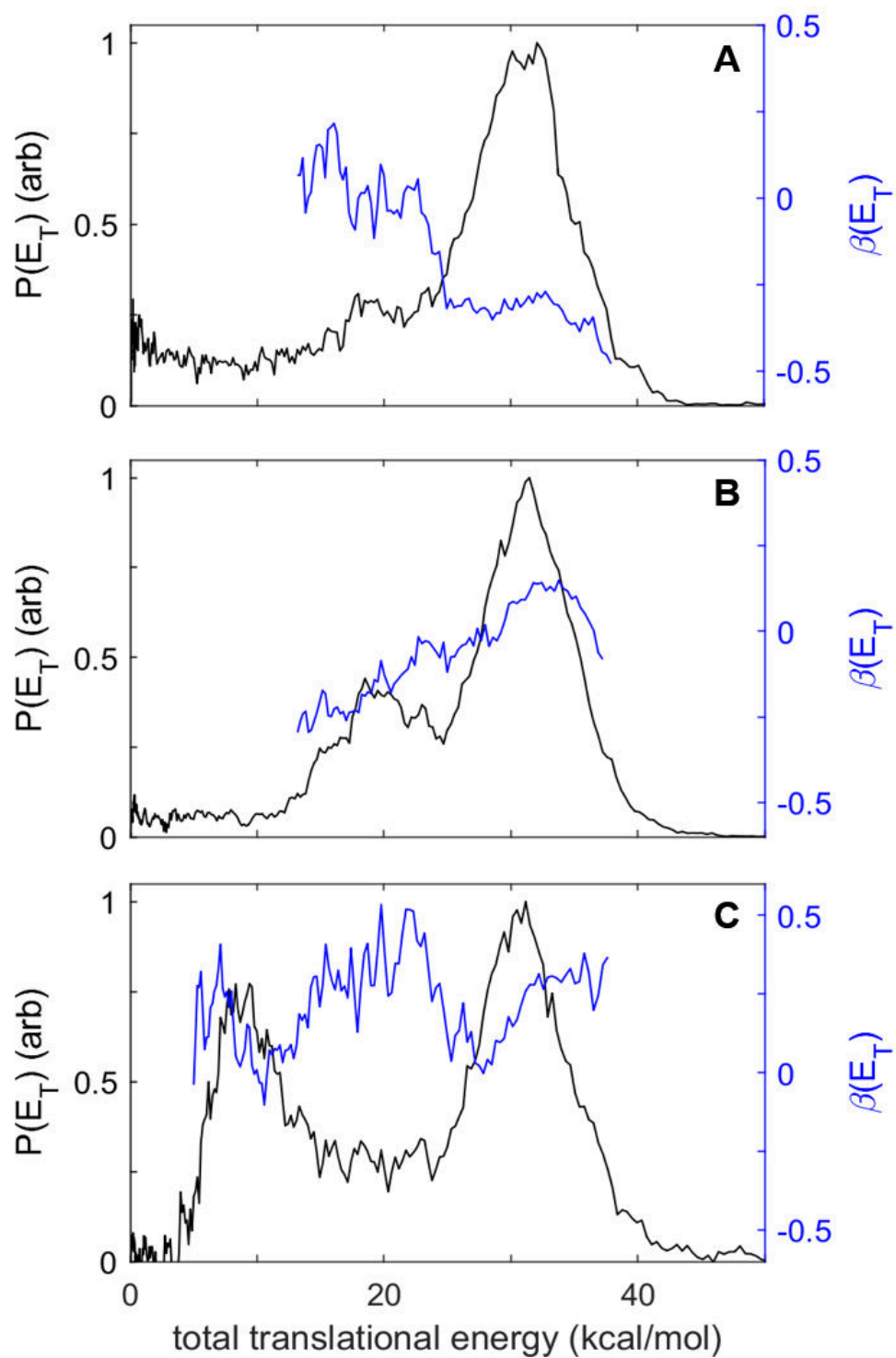
Fig. 3.5 Translational energy distributions (black) and anisotropy parameter \beta (blue) of Cl (A) Cl* (B) and C 3 H 3 (C) from photodissociation of propargyl chloride near 212 nm.
