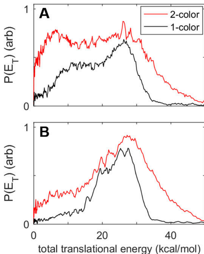
Fig. 4.2 Translational energy distributions of Cl (A) and Cl* (B) from 1-color UV (black) and 2-color (red) photodissociation of propargyl chloride photodissociation.
