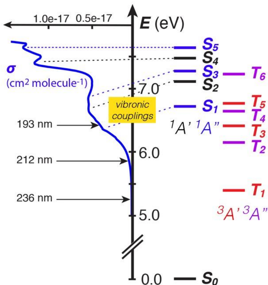
Fig. 3.6 Absorption spectrum of propargyl chloride (left, blue) at 295 K (adapted from Fahr et al.) and excitation energies of the singlet and triplet states located below 8 eV ( 3 \times {}^1A' (black), 3 \times {}^1A'' (blue), 3 \times {}^3A' (red), 3 \times {}^3A'' (purple),) calculated at the MRCI-F12/aug(Cl)-cc-pVTZ level. Laser excitation wavelengths are shown with black arrows and a tentative assignment of the features observed in the experimental spectrum with dashed lines. Note that strong vibronic couplings are expected for excitations to the S_1 , S_2 , S_3 , and S_4 states due in part to the presence of double-wells along the low-frequency CCC bending coordinate (see Fig. 3.7).
