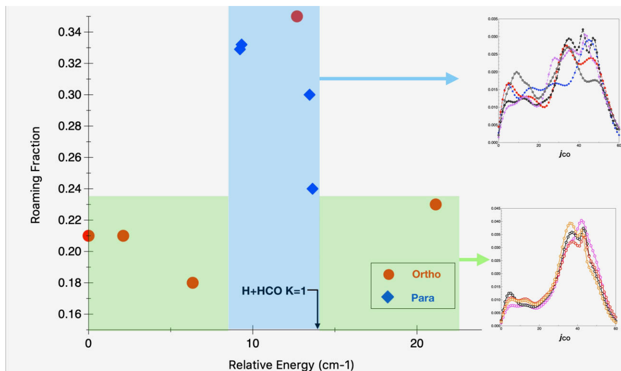
Fig. 6.12 Relative energy vs roaming fractions for ortho (red circles) and para transitions (blue diamonds). The region where a resonance between \text{H}_2\text{CO} and \text{H} + \text{HCO} states is observed is indicated by the blue box, with associated CO rotational distributions. Other ortho transitions (green box) and associated CO rotational distributions are also included.
