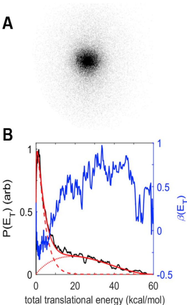
Fig. 4.6 DC slice image of HCl ( v = 0, j = 1 ) (A) and translational energy distribution (black) and anisotropy parameter b (blue) (B) from 2-color photodissociation of propargyl chloride. Red lines show decomposition of the distribution to two components (see text).
