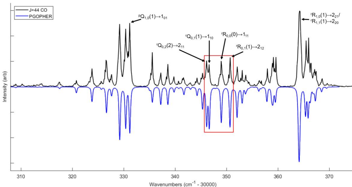
Fig. 6.1 2^14^3 PHOFEX spectrum with j_{\text{CO}} = 44 REMPI detection (top) and PGOPHER simulation (bottom). Commonly used ortho rotational lines and the four para rotational lines are labeled.
