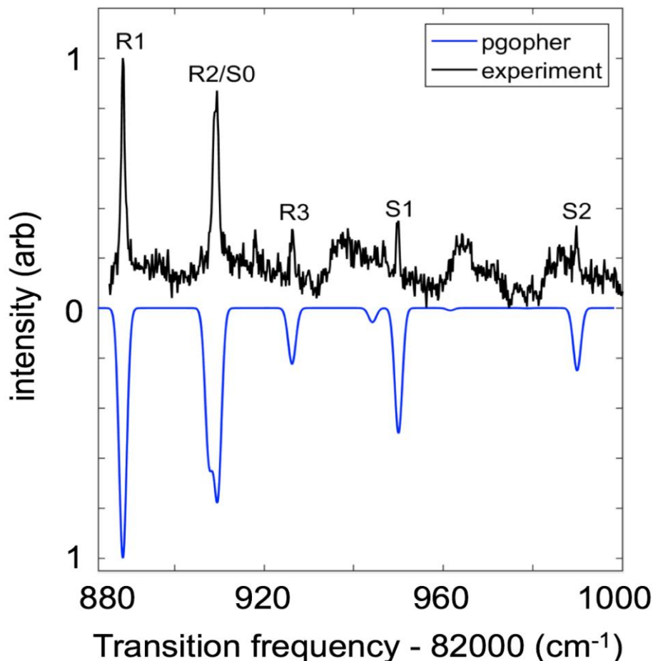
Fig. 4.5 Experimental HCl IRMPD REMPI spectrum (top trace) and simulation at 85 K (bottom trace).
