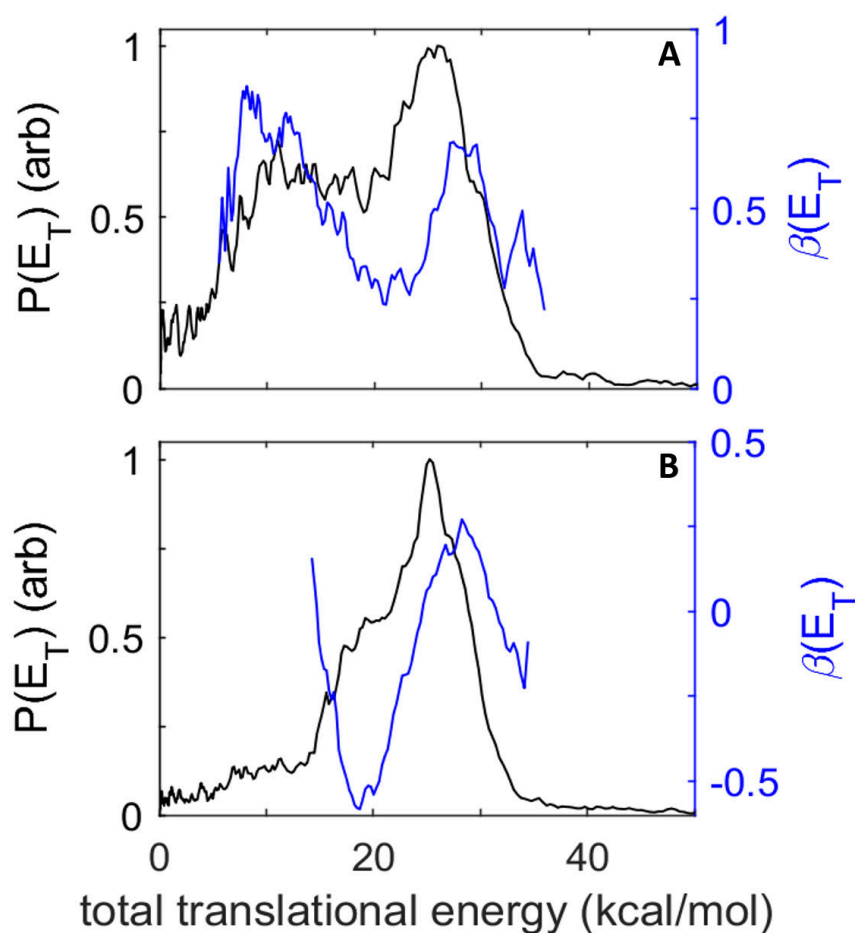
Fig. 3.3 Translational energy distributions (black) and anisotropy parameter \beta (blue) of Cl (A) and Cl* (B) from photodissociation of propargyl chloride near 236 nm.
