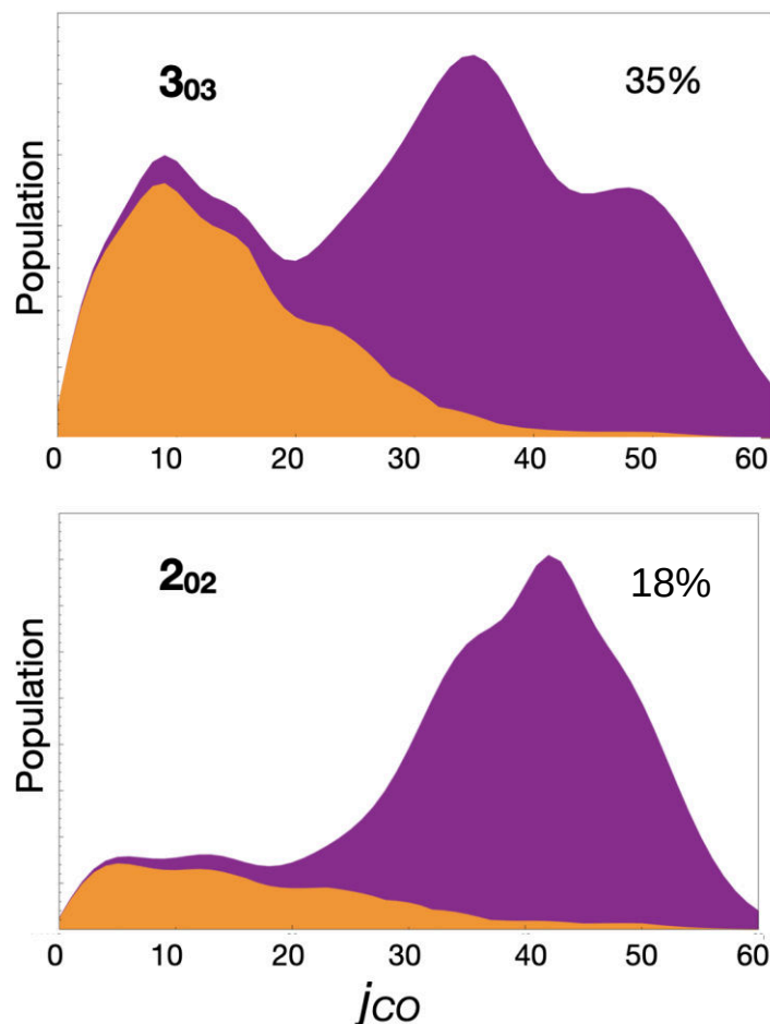
Fig. 6.9 Roaming fraction (orange) relative to the overall CO rotational distribution (purple) for 3_{03} (top) and 2_{02} (bottom) on 2^14^3 .
