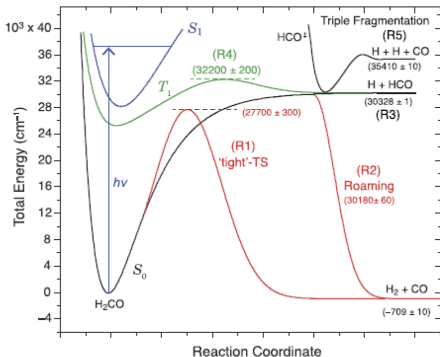
Fig. 5.1 Schematic of relevant PES cuts with energies and pathways indicated. Adapted with permission from M.S. Quinn et al, J. Chem. Phys. , 147, 013935 (2017) © AIP.
