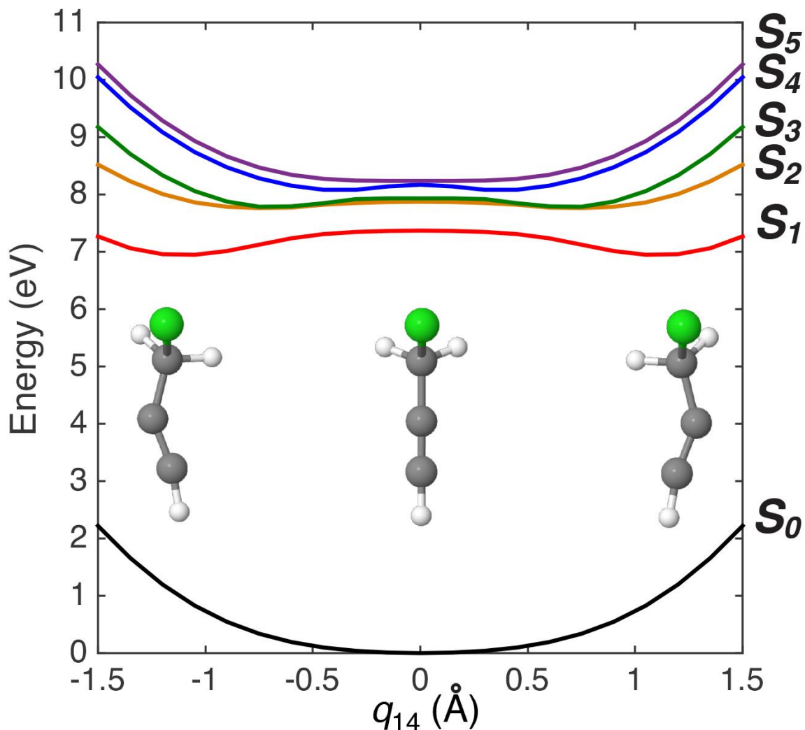
Fig. 3.7 Potential energies of the ground state S_0 and the five first singlet excited states calculated at the SA6-CASSCF(10/9)/cc-pVTZ level along the q_{14} normal mode.
