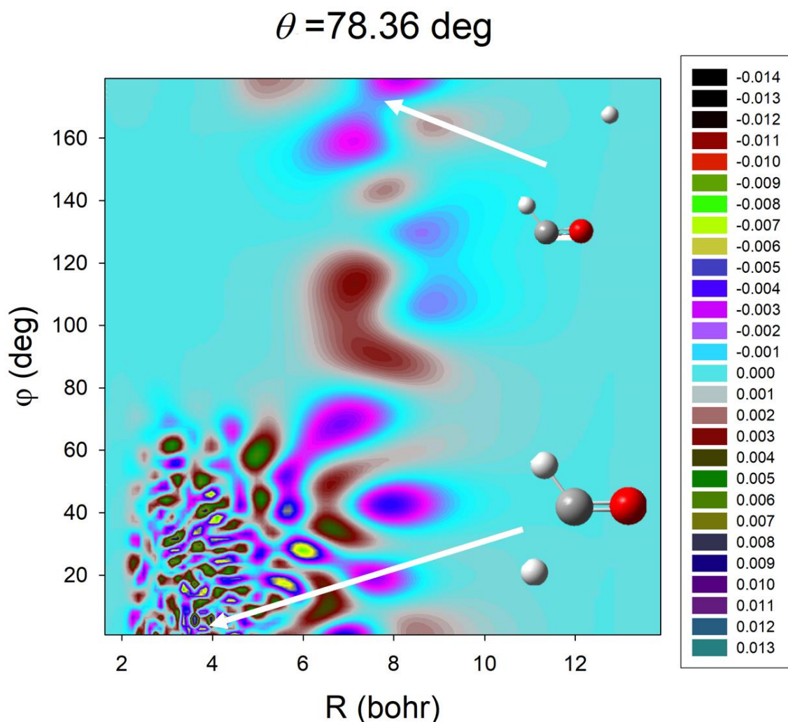
Fig. 6.15 Wavefunction near the radical threshold shown for dihedral angle of 78^\circ . Tight TS and roaming saddle point structures are marked.
