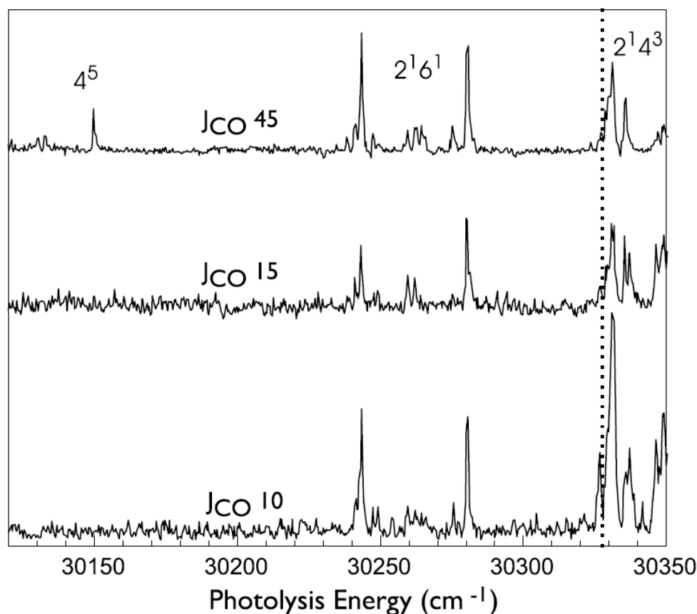
Fig. 1.4 PHOFEX spectra of different j_{\text{CO}} used to approximate the roaming onset. Adapted with permission from S.A. Lahankar et al, Chem. Phys. , 347, 288–299 (2008) © Elsevier.
