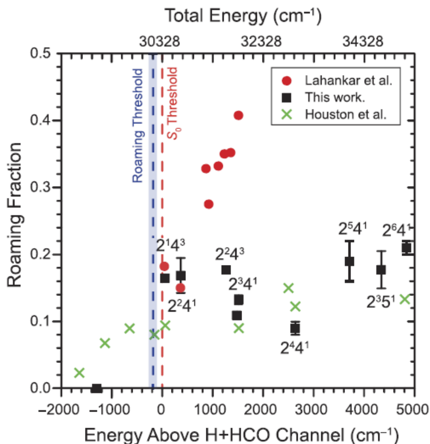
Fig. 1.5 Roaming channel branching fractions from CO ( v = 0 ) from Lahankar, Sutis, and coworkers (red dots), Kable and coworkers (black dots), and a quasiclassical trajectory study. Adapted with permission from M.S. Quinn et al, J. Chem. Phys. , 147, 013935 (2017) © AIP.
