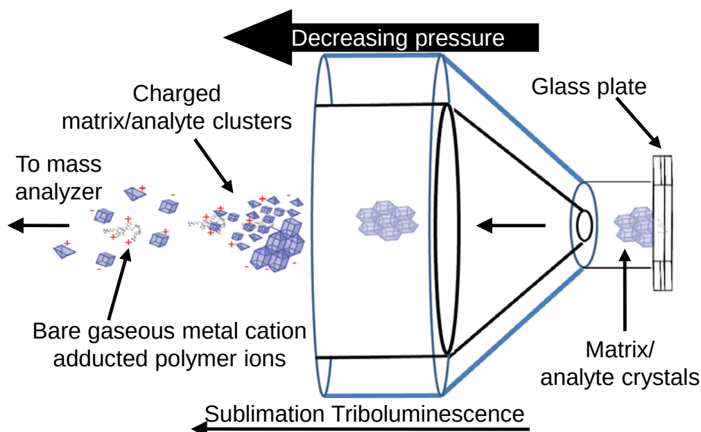
Scheme 1: Schematic of the processes associated with MAI, here shown using the glass plate introduction method directly from atmospheric pressure using a modified skimmer inlet.
