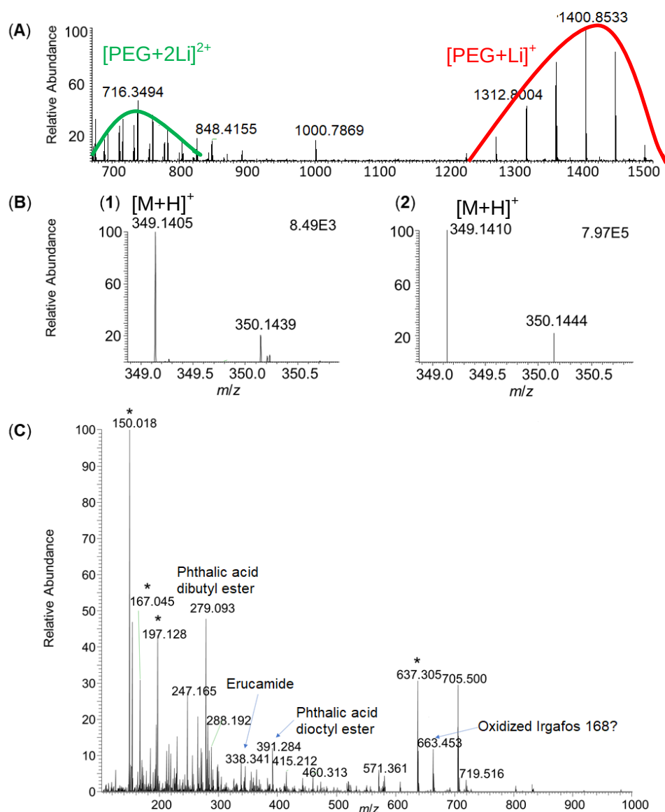
Figure 7. Accurate mass measurements on an uncalibrated mass spectrometer using the matrix 3-NBN: (A) PEG-1500 ionized in the presence of lithium chloride, (B) plasticizer bisphenol A (1) experimental and (2) modeled isotopic distribution, and (C) packing material extracted with acetone. Asterisks mark peaks associated with the matrix 3-NBN. Data acquired using the dedicated vacuum source on a Thermo Q-Exactive Focus.
