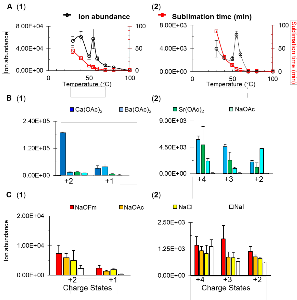
Figure 3. Ion abundance and sublimation time using the MAI matrix 2-methyl-2-nitro-1,3-propanediol and the role of (A) temperature using Ba(OAc) 2 , (B) cation acetates, and (C) sodium counter anions, respectively, used for ionization of (1) PEG-1000 and (2) PEG-3000 on a Waters SYNAPT G2 mass spectrometer (Scheme S1B, Movie S1) using a source block temperature of 55 °C. For more details, refer to Figure S13.
