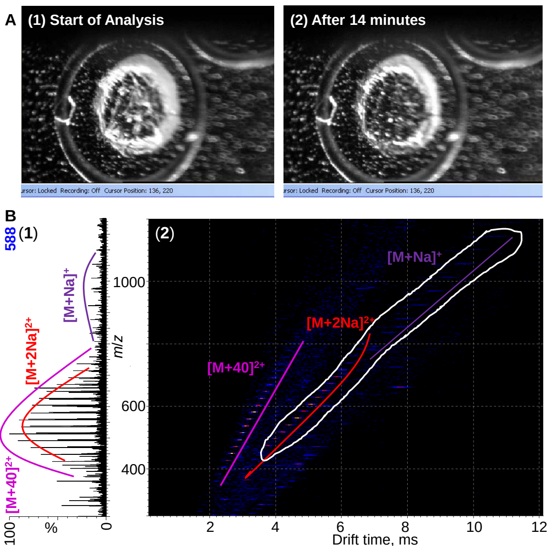
Figure 2. MAI-IMS-MS of linear PEG with bronopol matrix using an intermediate pressure MALDI source without the use of a laser: (A) screenshot commercial sample plate in the vacuum region of the source used to monitor the spontaneous ionization process without the addition of energy (1) at the beginning and (2) end of acquisition, (B) ions detected and displayed by (1) total mass spectrum and (2) IMS-MS 2-dimensional plot of drift time versus m/z . For more details, refer to Figure S7 and S8 .
