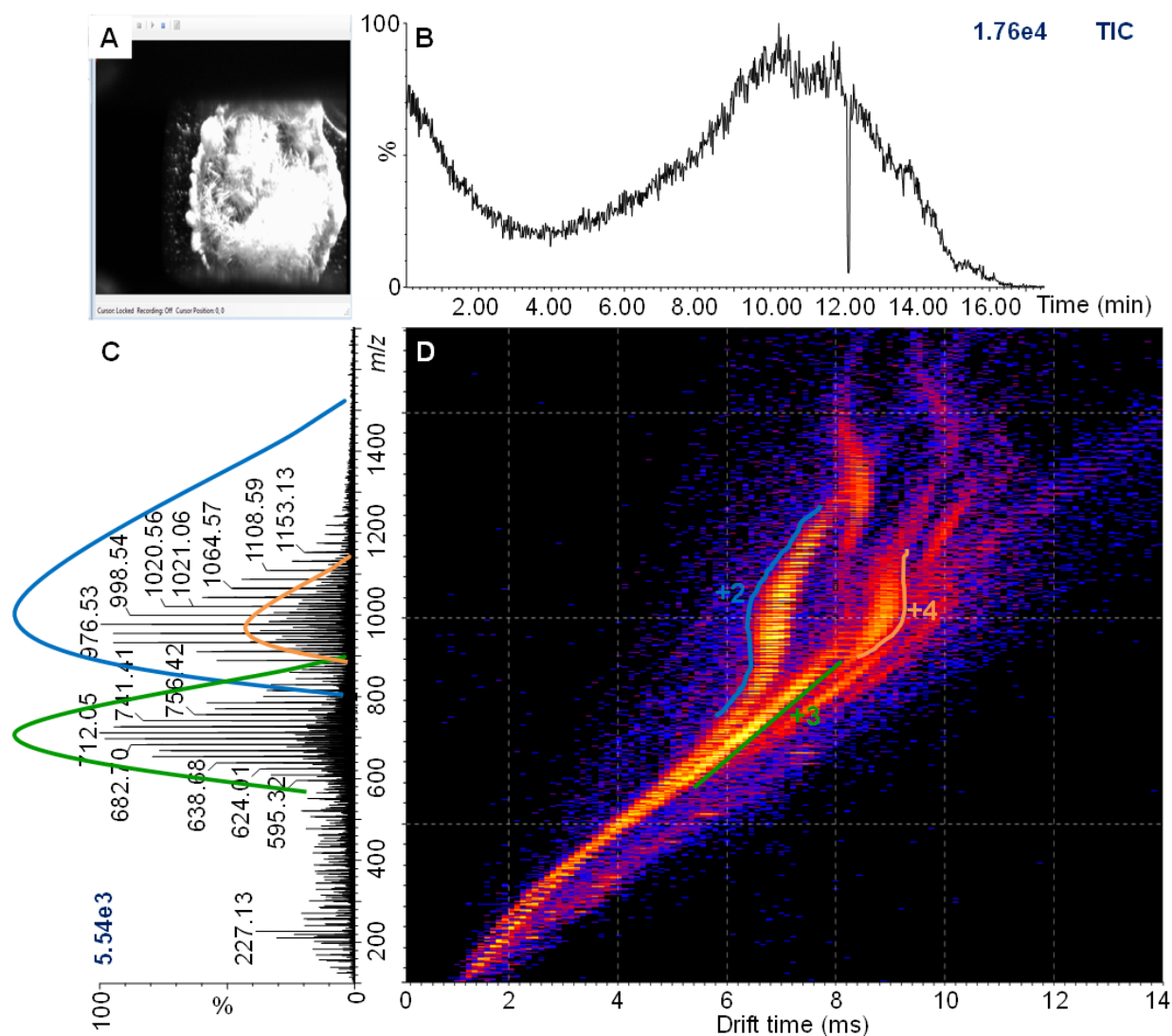
Figure 1. MALDI-IMS-MS of PEG-DME 2000 doped with LiTFA (9:1 v/v ratio) with 3-NBN matrix: (A) screenshot of the crystallized PEG-DME 2000:LiTFA (1 \mu L) and 3-NBN matrix (1 \mu L) on the sample metal plate, (B) total ion chromatogram, (C) total mass spectrum and (D) 2-dimensional plot of drift time versus m/z showing the +4, +3 and +2 charge states. Data acquired using MALDI settings on the intermediate pressure MALDI source of Waters SYNAPT G2S mass spectrometer. For more details, refer to Figure S6 .
