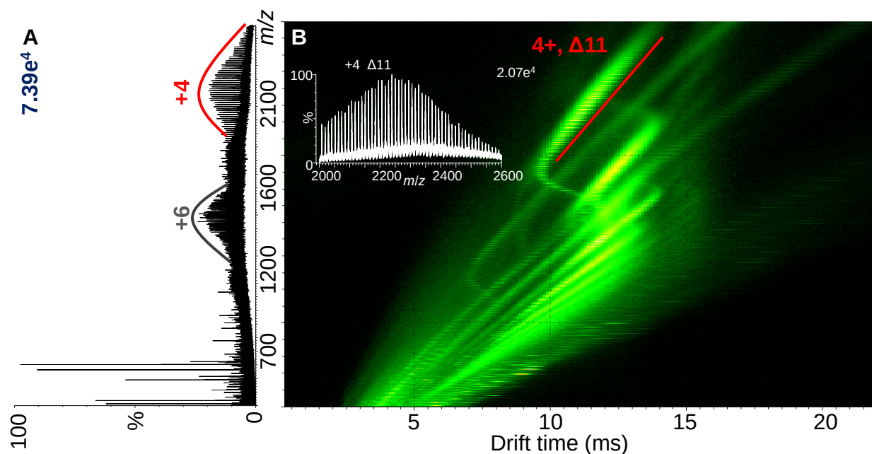
Figure 4. vMAI-IMS-MS of PEG-10000 and calcium II acetate salt in a 1:100 molar ratio and 2-methyl-2-nitropropane-1,3-diol matrix: (A) total mass spectrum and (B) 2-D plot display of drift time versus m/z with inset of the extracted +4 charge state. Data acquired on a Waters SYNAPT G2 mass spectrometer ( Scheme S1B , Movie S1 ). For more details, refer to Figure S14 .
