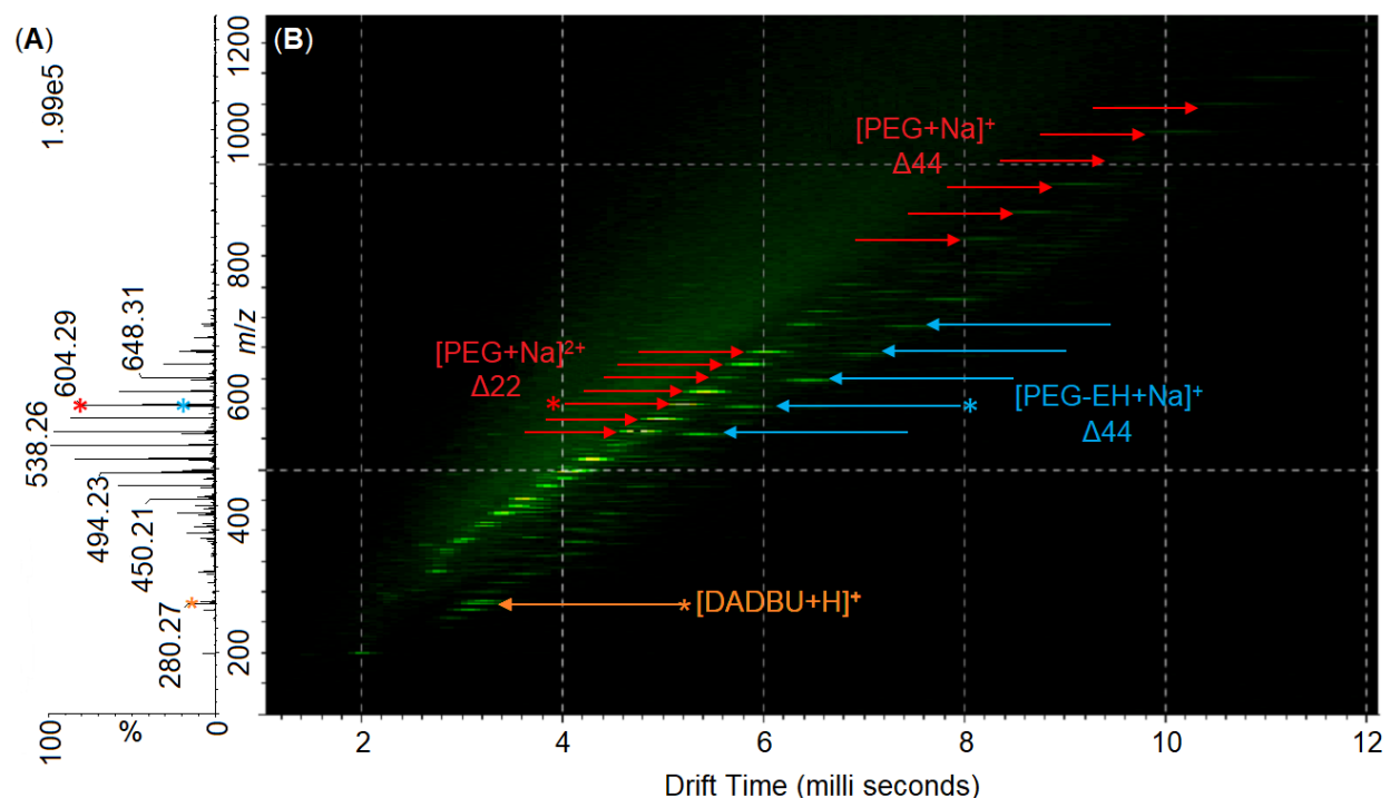
Figure 8. vMAI-IMS-MS approach to the analysis of a tertiary mixture containing a polymer, plasticizer, and property modifier. (A) total mass spectrum and (B) 2-D plot of drift time versus m/z containing PEG-1000 (red), plasticizer PEG-EH 640 (blue), and property modifier DADBU (yellow). Data acquired with vMAI using 3-NBN matrix and NaTFA salt on the vacuum-probe 70 fitted on a Waters SYNAPT G2S. For reference, colored asterisks match signal in 2D plot of drift time versus m/z with the corresponding peak in the mass spectrum. For more details, refer to Figure S27 .
