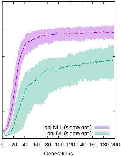
friction_dyn_one-hot
