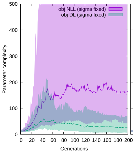
friction_dyn_one-hot
