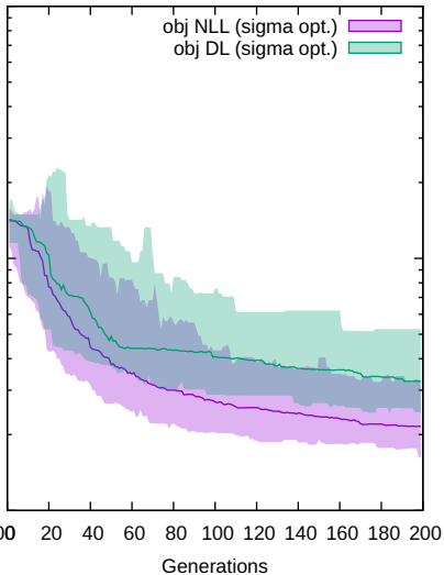
friction_dyn_one-hot
