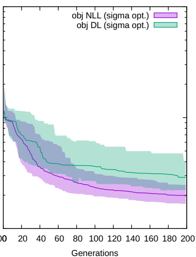
friction_dyn_one-hot
