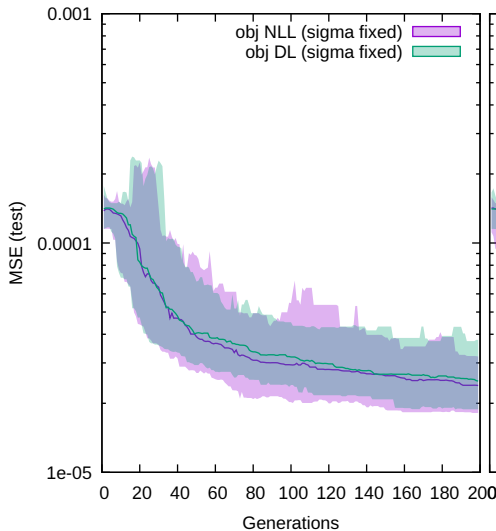
friction_dyn_one-hot
