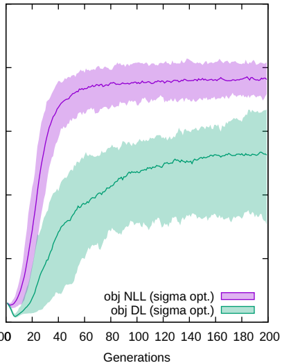
friction_stat_one-hot
