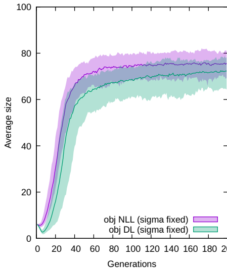
friction_dyn_one-hot
