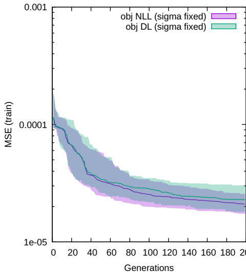
friction_dyn_one-hot
