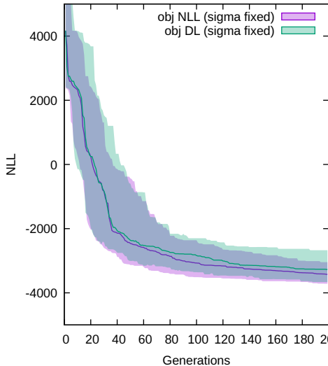
friction_dyn_one-hot
