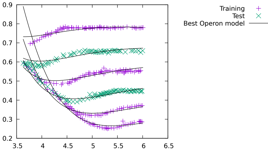
Nikuradse 1 Best Operon Solution
