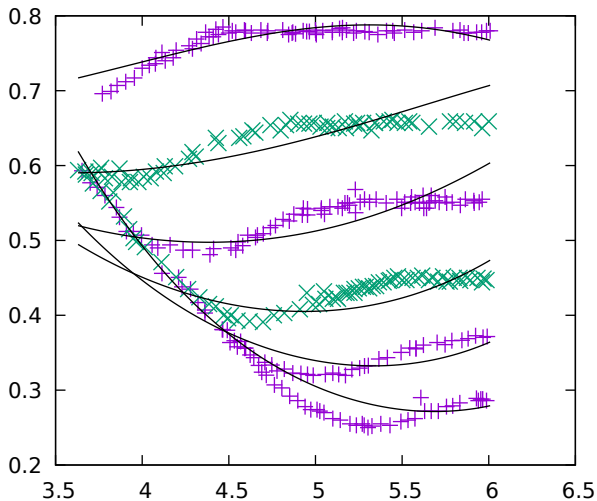
Nikuradse 1 Best EggMo Solution
