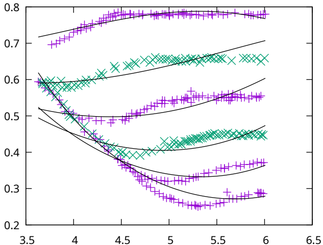
Nikuradse 1 Best EggMo Solution
