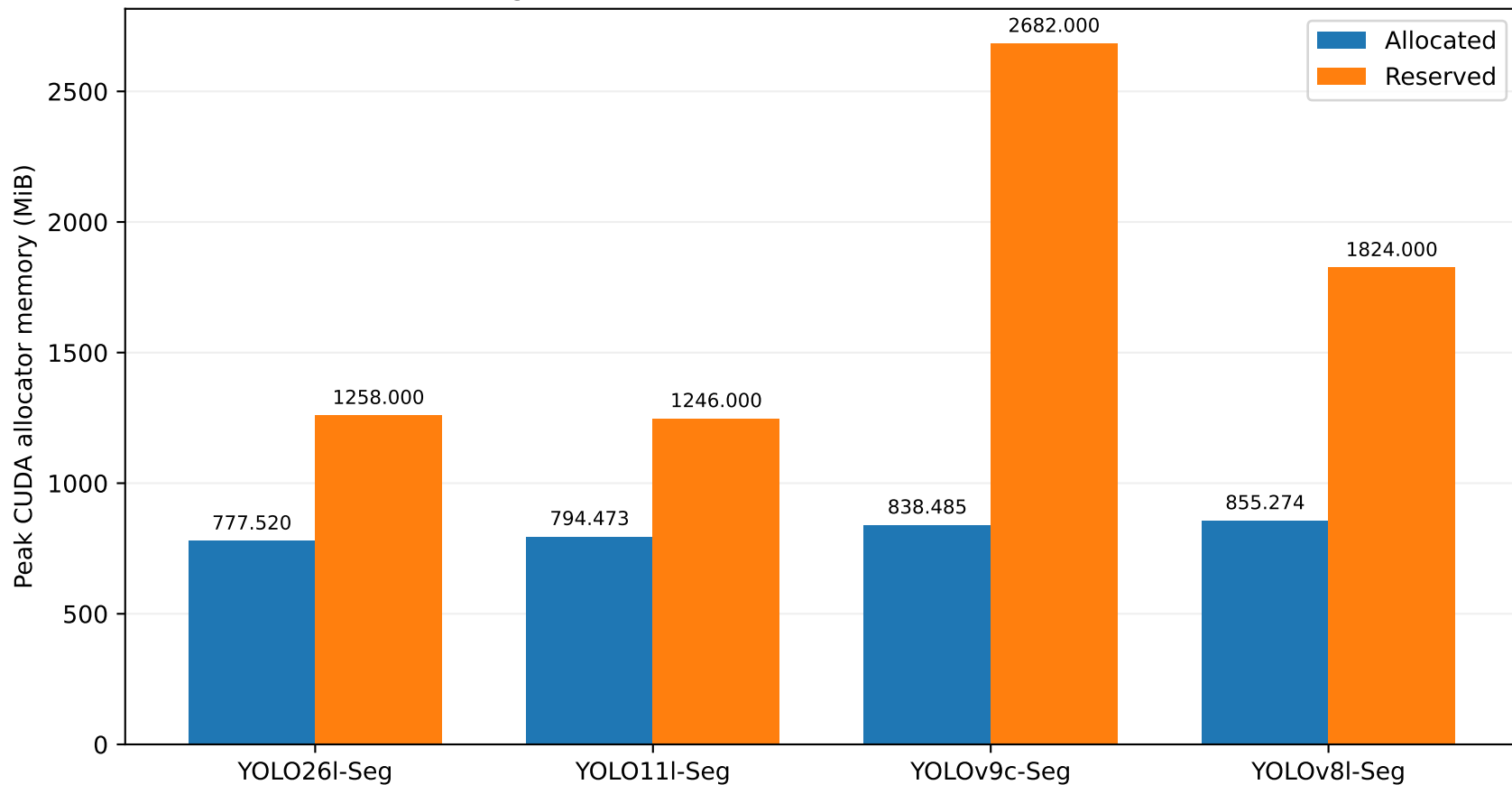
Second-largest available variants • MOTS20 Person • FP32 / 640
