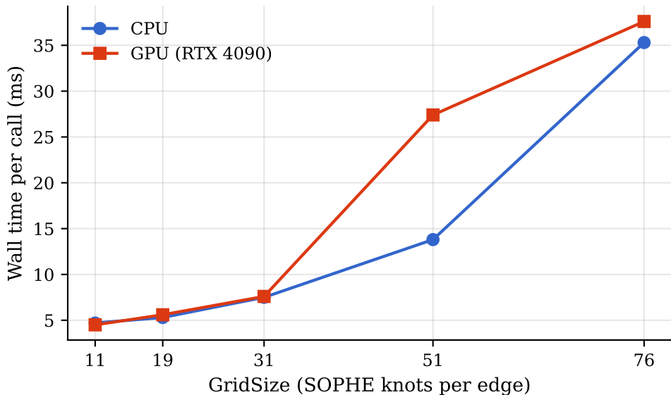
pepper() single-call latency ( S=1/2 + {}^1\text{H} )
