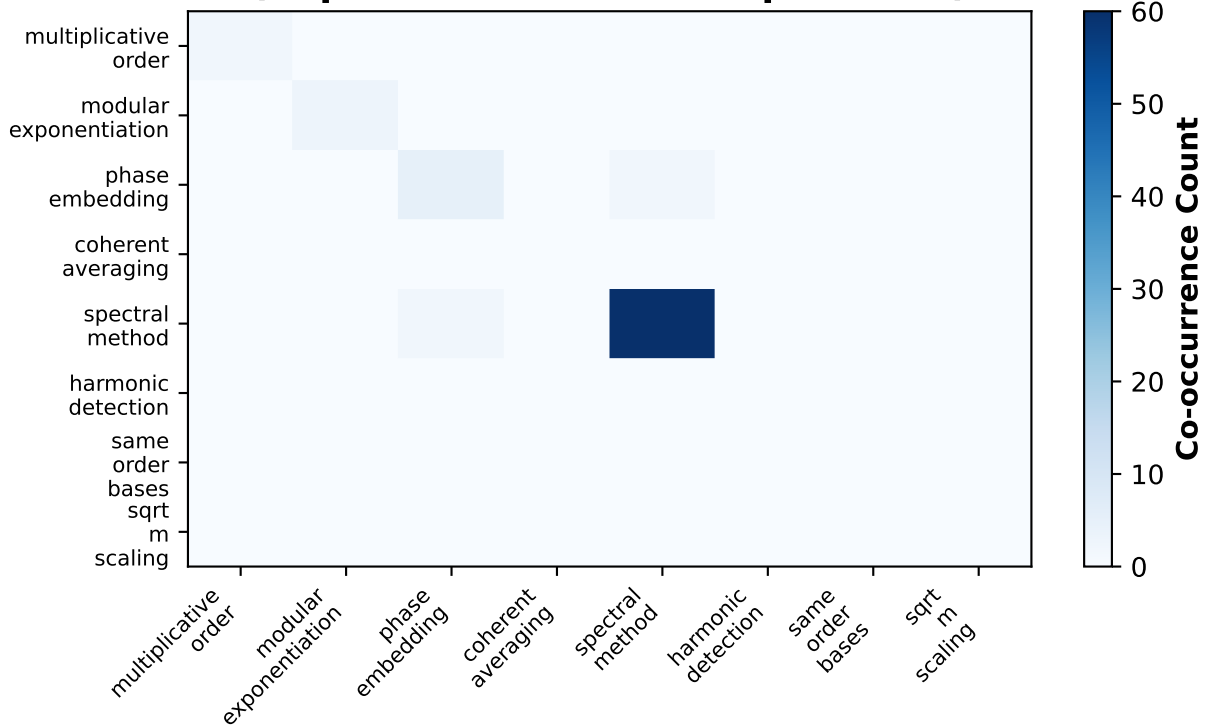
Concept Co-occurrence Matrix (Papers with both concepts > 0.2)
