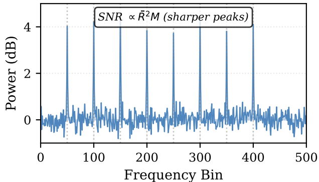
VRA Coherent Averaging
