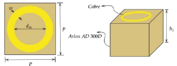
Figure 5.- Representation of the FSS unite-cell, where "P" is the periodicity, "din" is the inner diameter, and "w" is the broad of the ring.
