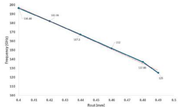
Figure 9.- Tendencia of the displacement of the frequency versus the increase of the radius where the dashed line is the trend.
