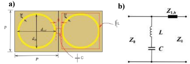
Figure 4.- a) Schematic representation of two unit cells that form an FSS with ring-type elements, where the rings are modeled as the inductive part (L) and the distance between elements as the capacitive part (C). b) Equivalent circuit of the FSS.
