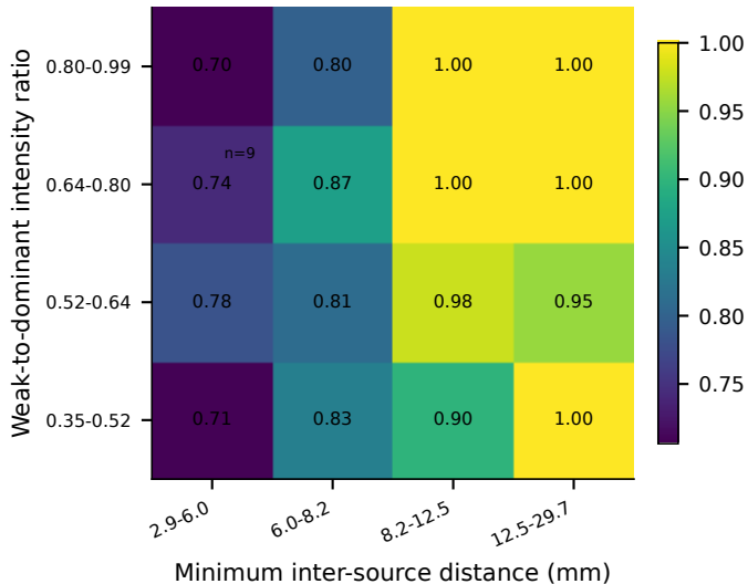
(a) SSQ-FMT Component Recall
