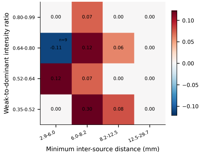
(b) Merge Probability Reduction vs. No Source Cue
