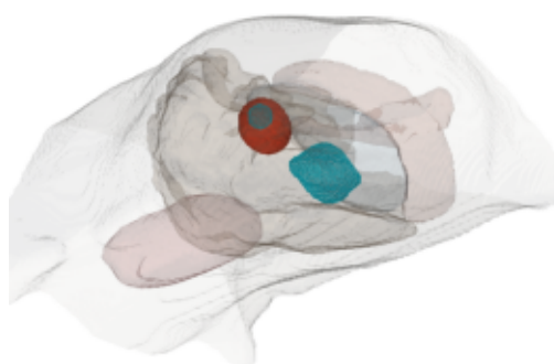
(a) Weak secondary focus 2 foci | irregular + sphere
