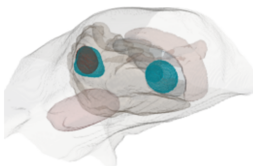
(c) Mixed morphology 3 foci | ellipsoid + irregular + sphere
