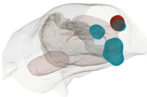
(b) Adjacent-source merging 3 foci | ellipsoid + irregular
