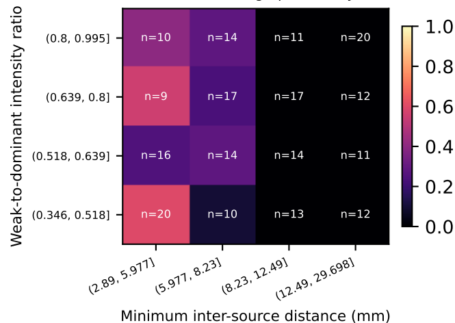
Merge reduction vs w/o source-relative query cue
