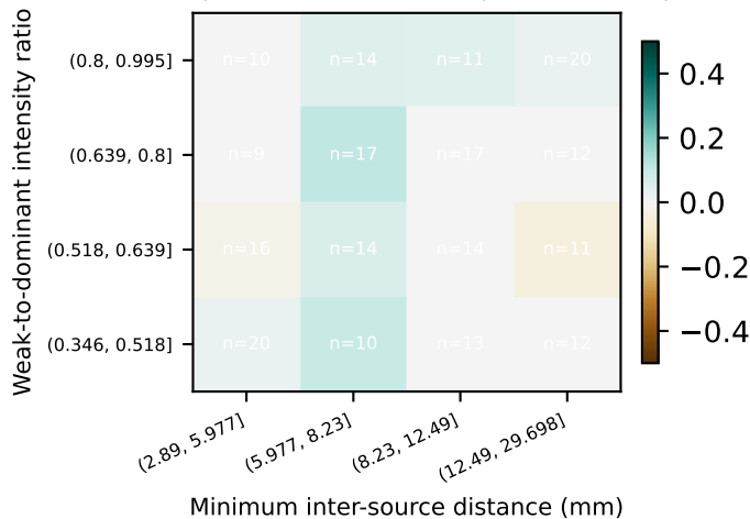
Recall improvement vs w/o transport-aware footprint
