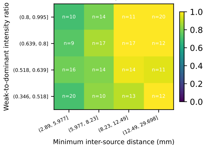
Recall improvement vs w/o transport-aware footprint
