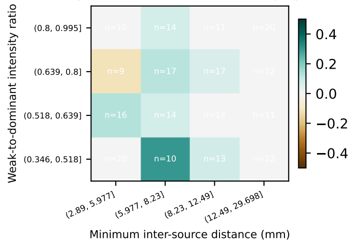
Merge reduction vs w/o source-relative query cue
