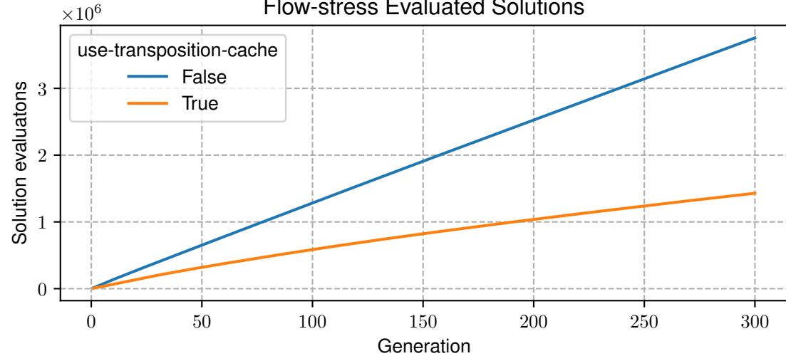
Flow-stress Evaluated Solutions
