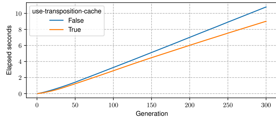
Flow-stress Mean Runtime
