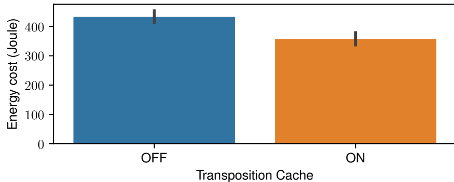
Gradient descent iterations: 100 (energy savings = 23.8%)
