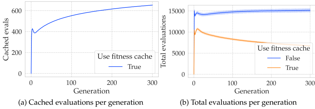
Figure 8: Cached and total evaluations per generation. The shaded regions represent the 95% confidence intervals.
