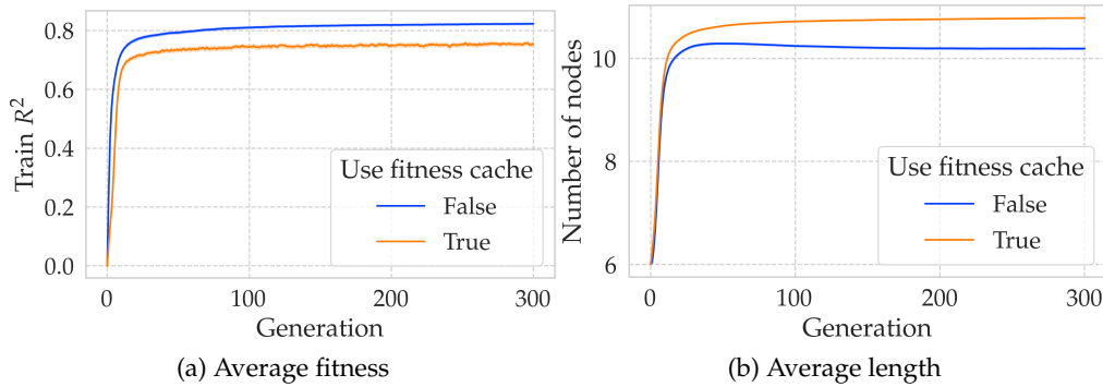
Figure 7: Average fitness and length, with/without caching. The shaded regions represent the 95% confidence intervals.
