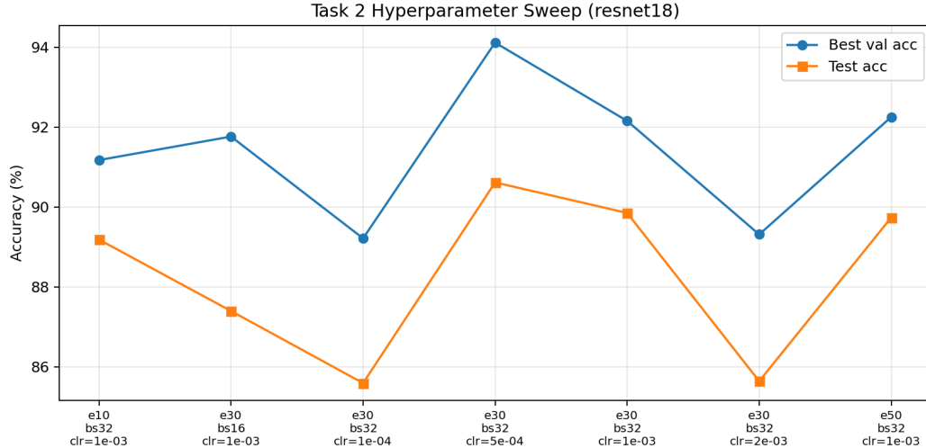
Figure 2: Task 2 ResNet-18 hyperparameter sweep. Each tick shows epochs, batch size, and classifier learning rate.
