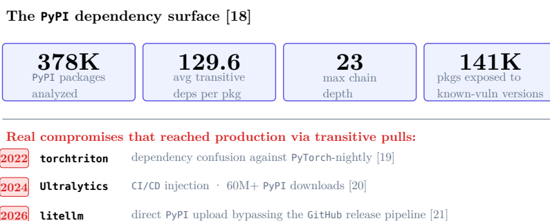
Figure 5: Top: ecosystem-level statistics on the transitive-dependency surface from [18]. Bottom: three real compromises that reached production ML stacks via transitive pulls in 2022–2026.
