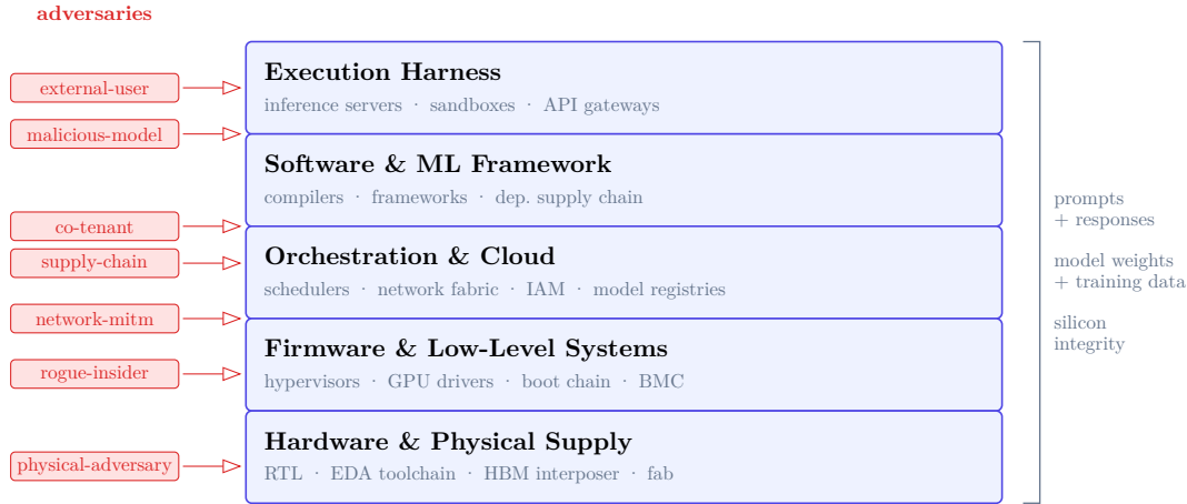
Figure 2: The five layers of the ML inference and training stack, with the adversary archetypes (left) that each layer invites and the assets (right) that pass through them. Adversaries are tagged on each layer below using the same labels; see Section 4 for full descriptions.
