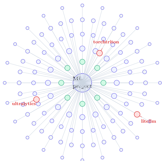
Figure 5: The transitive-dependency surface of a typical ML project. Direct dependencies (inner green ring) pull in cascading transitive deps to a measured maximum depth of 23 [17]. Red nodes are real 2022-26 compromises ( torchtriton , ultralytics , litellm ) that reached production through indirect pulls.
