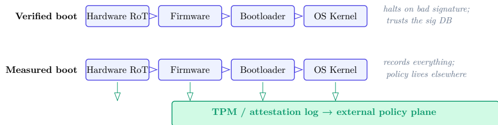
Figure 7: Two strategies for boot-chain integrity. Verified boot halts on a bad signature at each stage but trusts whatever lives in the signature database. Measured boot records hashes into a TPM and defers enforcement to an external policy plane that can release secrets, quarantine, or hard-reset based on attestation.
