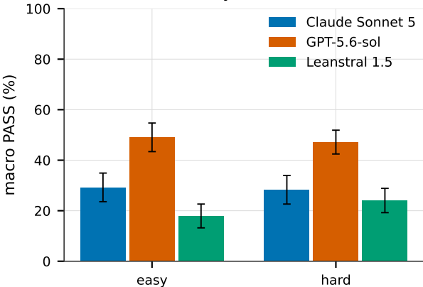
macro PASS by model and mode
